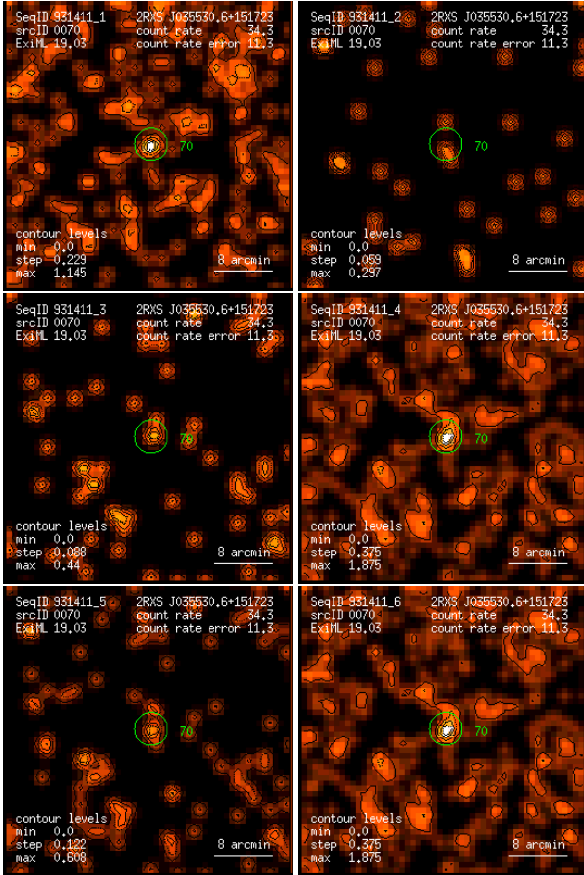
Figure 70: RASS 931411: detection 0070: band rate images, Gaussian filter: (1) PSPC channels 11 – 41, (2) 52 – 90, (3) 91 – 201, (4) 11 – 235, (5) 52 – 201, (6) 11 – 201. Broad band rates in counts/ks. Band rate contour levels in counts/ks/arcmin 2 .
