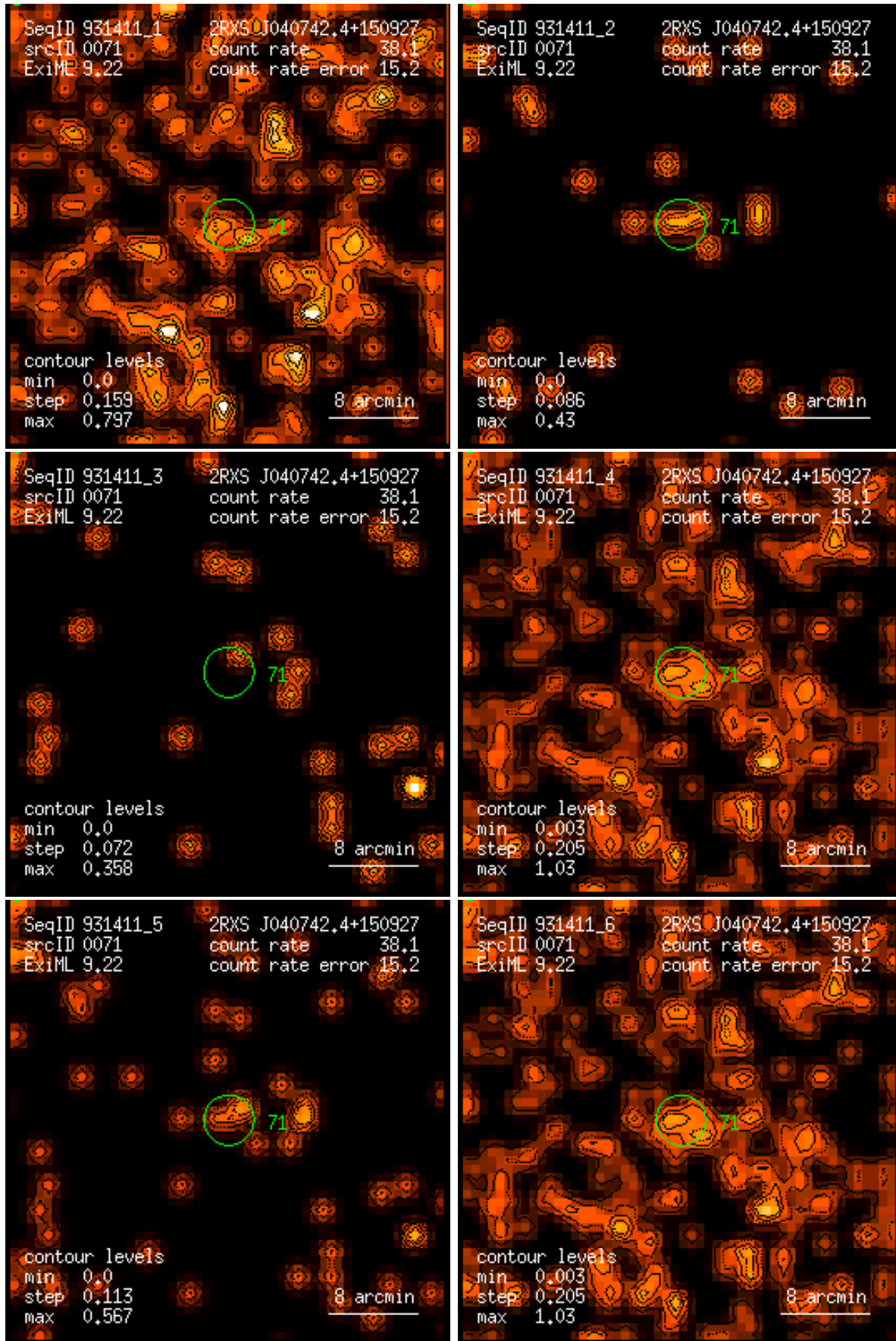
Figure 71: RASS 931411: detection 0071: band rate images, Gaussian filter: (1) PSPC channels 11 – 41, (2) 52 – 90, (3) 91 – 201, (4) 11 – 235, (5) 52 – 201, (6) 11 – 201. Broad band rates in counts/ks. Band rate contour levels in counts/ks/arcmin 2 .
