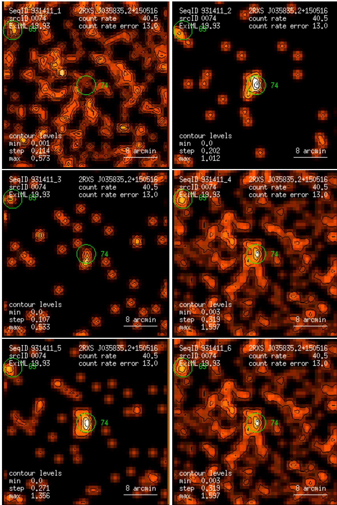
Figure 74: RASS 931411: detection 0074: band rate images, Gaussian filter: (1) PSPC channels 11 – 41, (2) 52 – 90, (3) 91 – 201, (4) 11 – 235, (5) 52 – 201, (6) 11 – 201. Broad band rates in counts/ks. Band rate contour levels in counts/ks/arcmin 2 .
