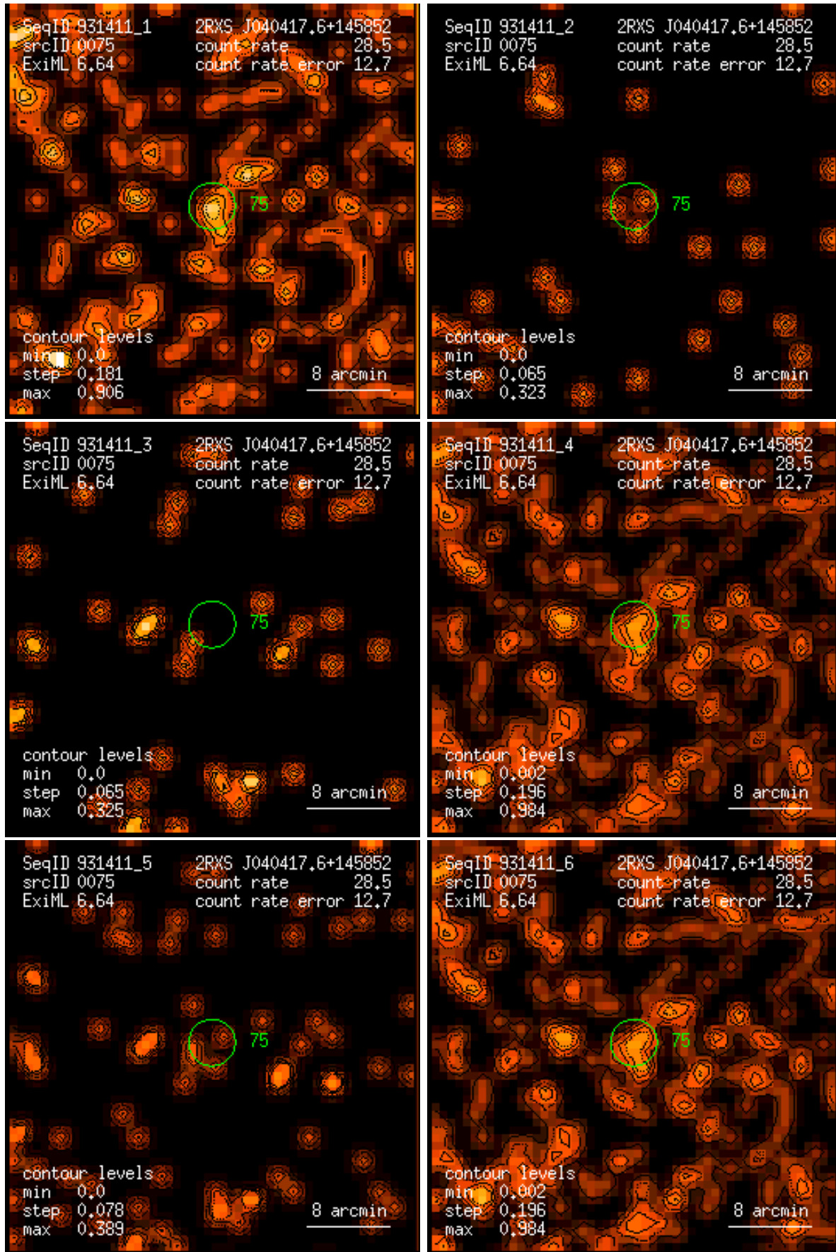
Figure 75: RASS 931411: detection 0075: band rate images, Gaussian filter: (1) PSPC channels 11 – 41, (2) 52 – 90, (3) 91 – 201, (4) 11 – 235, (5) 52 – 201, (6) 11 – 201. Broad band rates in counts/ks. Band rate contour levels in counts/ks/arcmin 2 .
