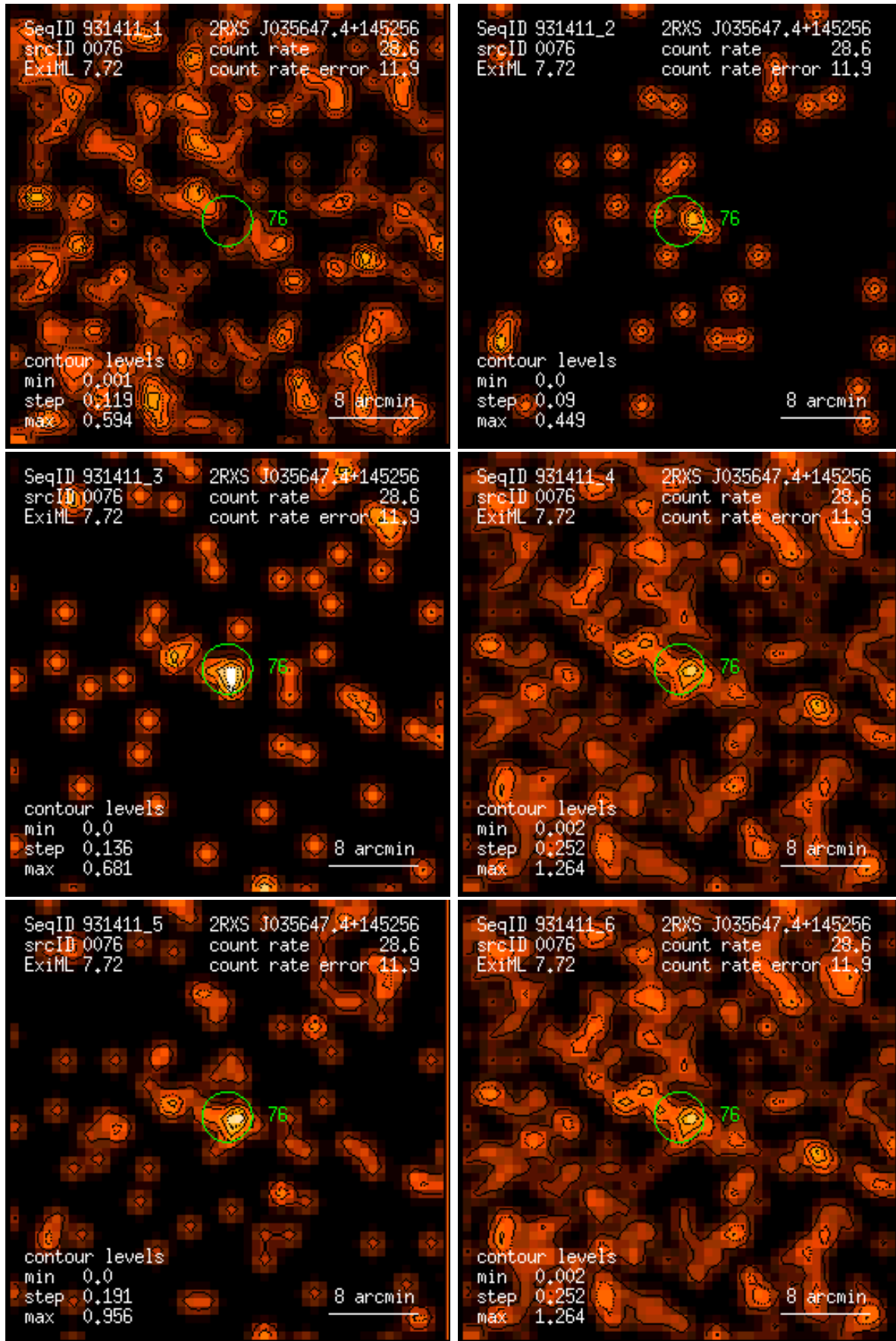
Figure 76: RASS 931411: detection 0076: band rate images, Gaussian filter: (1) PSPC channels 11 – 41, (2) 52 – 90, (3) 91 – 201, (4) 11 – 235, (5) 52 – 201, (6) 11 – 201. Broad band rates in counts/ks. Band rate contour levels in counts/ks/arcmin 2 .
