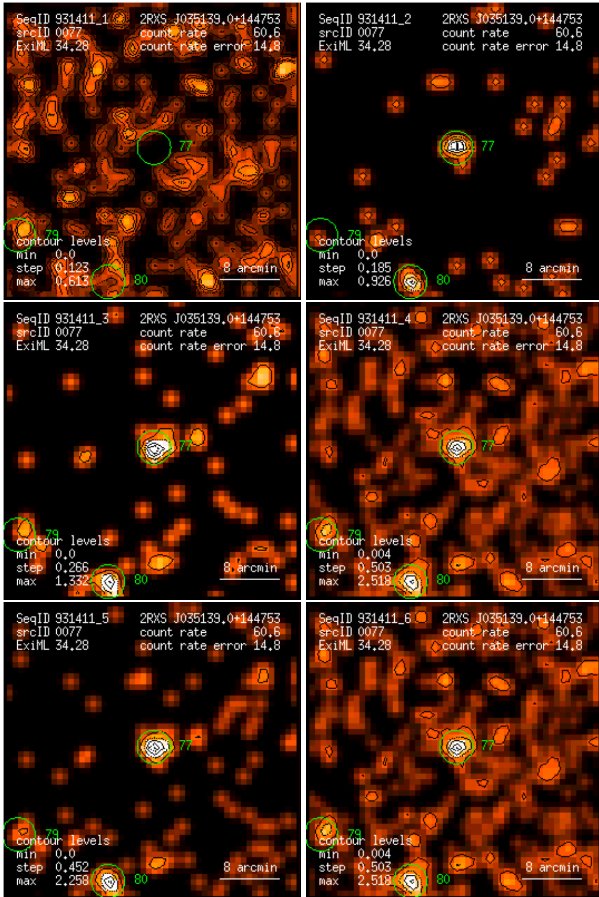
Figure 77: RASS 931411: detection 0077: band rate images, Gaussian filter: (1) PSPC channels 11 – 41, (2) 52 – 90, (3) 91 – 201, (4) 11 – 235, (5) 52 – 201, (6) 11 – 201. Broad band rates in counts/ks. Band rate contour levels in counts/ks/arcmin 2 .
