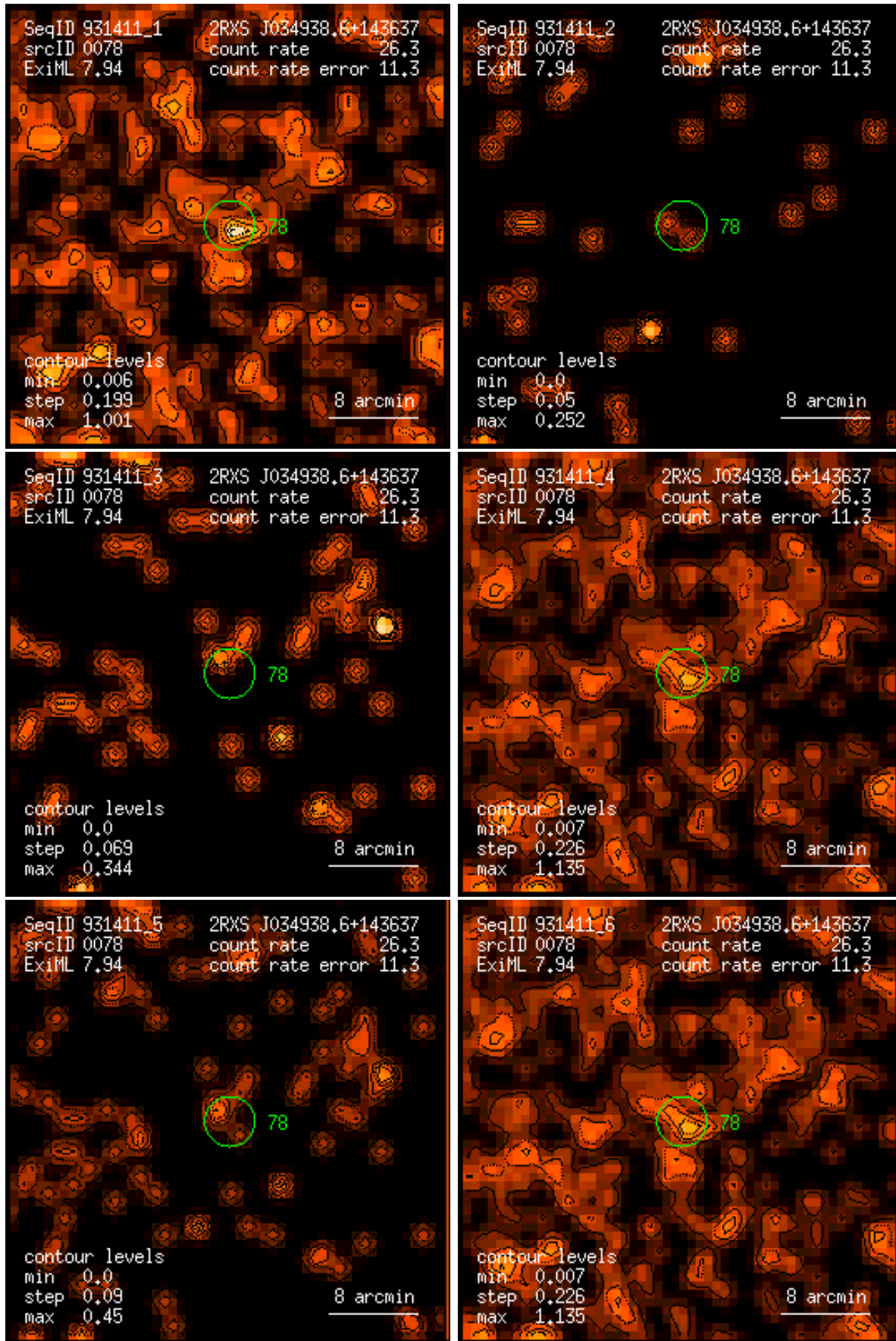
Figure 78: RASS 931411: detection 0078: band rate images, Gaussian filter: (1) PSPC channels 11 – 41, (2) 52 – 90, (3) 91 – 201, (4) 11 – 235, (5) 52 – 201, (6) 11 – 201. Broad band rates in counts/ks. Band rate contour levels in counts/ks/arcmin 2 .
