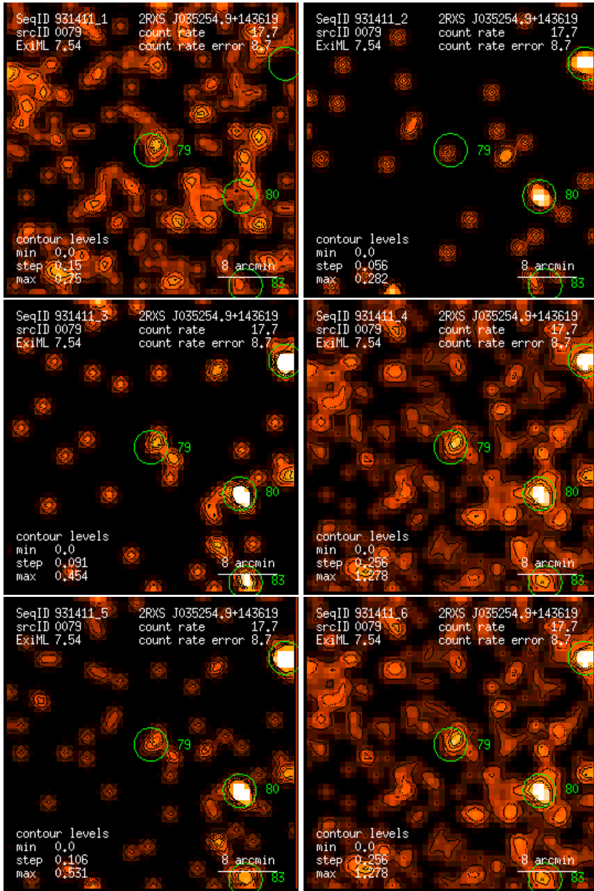
Figure 79: RASS 931411: detection 0079: band rate images, Gaussian filter: (1) PSPC channels 11 – 41, (2) 52 – 90, (3) 91 – 201, (4) 11 – 235, (5) 52 – 201, (6) 11 – 201. Broad band rates in counts/ks. Band rate contour levels in counts/ks/arcmin 2 .
