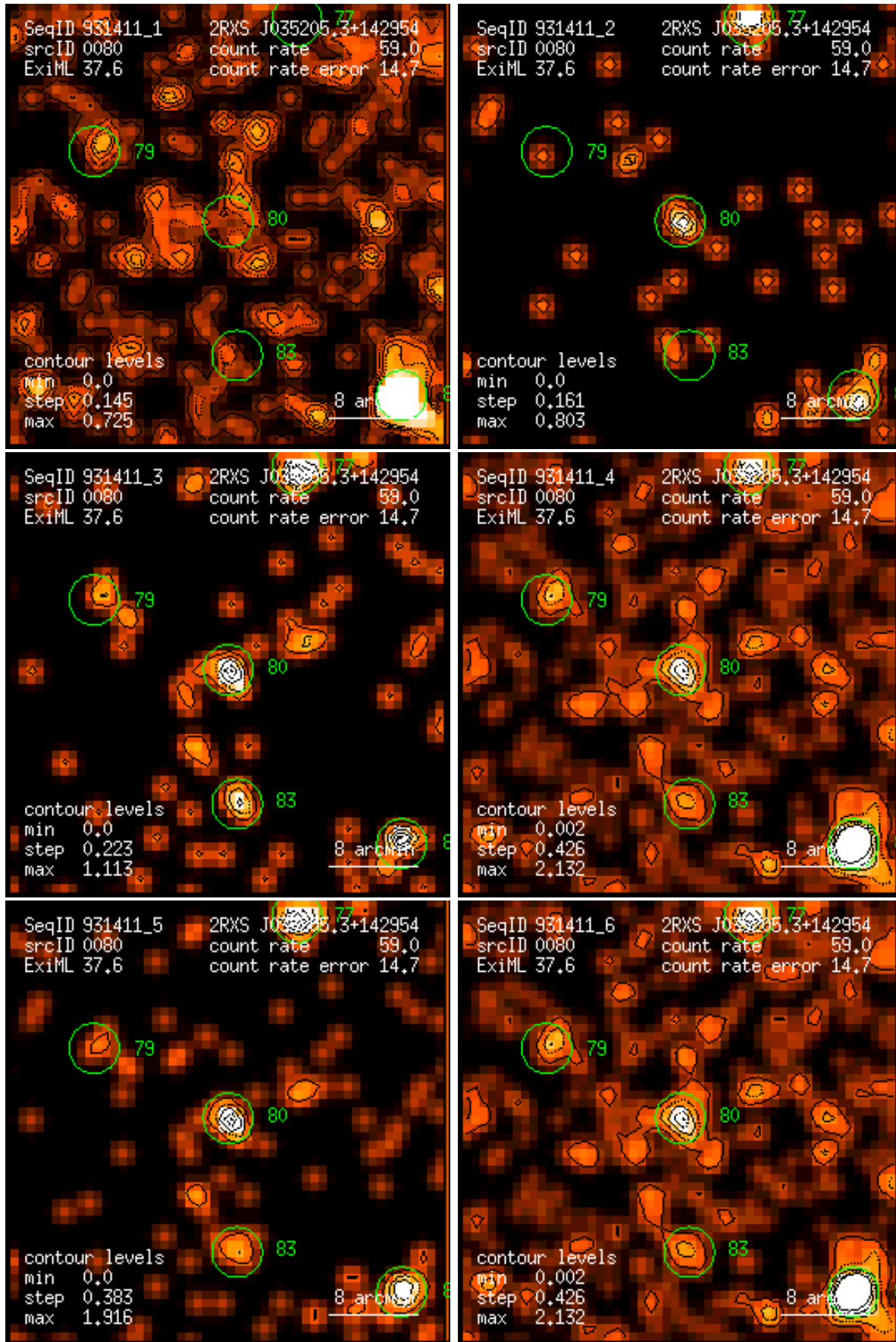
Figure 80: RASS 931411: detection 0080: band rate images, Gaussian filter: (1) PSPC channels 11 – 41, (2) 52 – 90, (3) 91 – 201, (4) 11 – 235, (5) 52 – 201, (6) 11 – 201. Broad band rates in counts/ks. Band rate contour levels in counts/ks/arcmin 2 .
