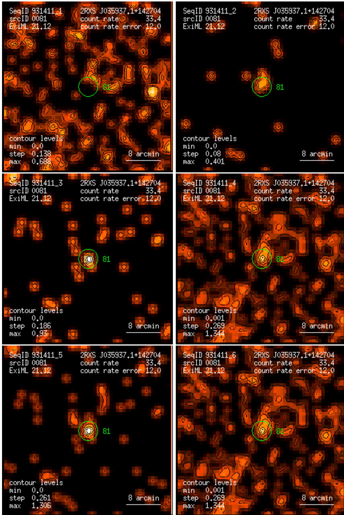
Figure 81: RASS 931411: detection 0081: band rate images, Gaussian filter: (1) PSPC channels 11 – 41, (2) 52 – 90, (3) 91 – 201, (4) 11 – 235, (5) 52 – 201, (6) 11 – 201. Broad band rates in counts/ks. Band rate contour levels in counts/ks/arcmin 2 .
