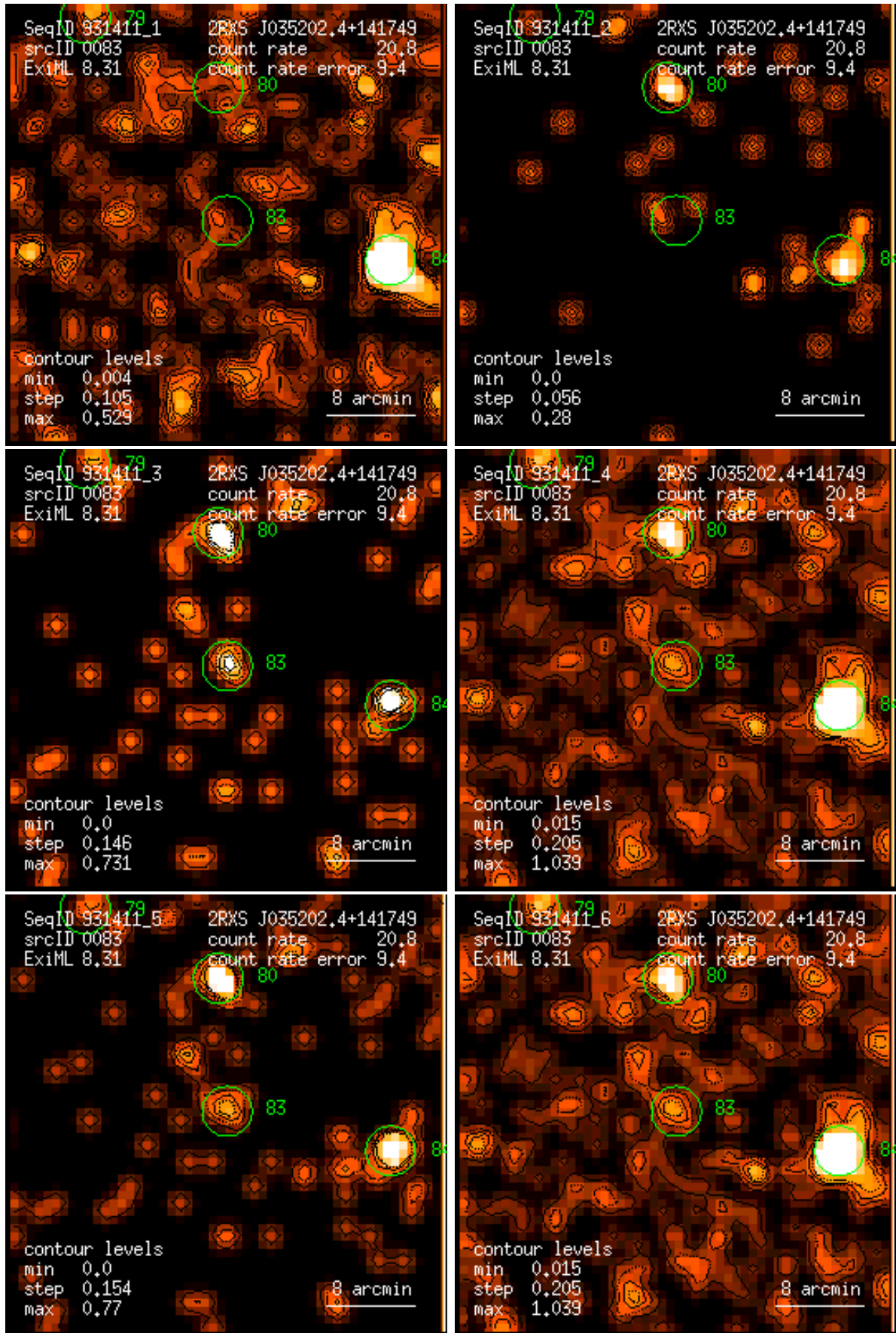
Figure 83: RASS 931411: detection 0083: band rate images, Gaussian filter: (1) PSPC channels 11 – 41, (2) 52 – 90, (3) 91 – 201, (4) 11 – 235, (5) 52 – 201, (6) 11 – 201. Broad band rates in counts/ks. Band rate contour levels in counts/ks/arcmin 2 .
