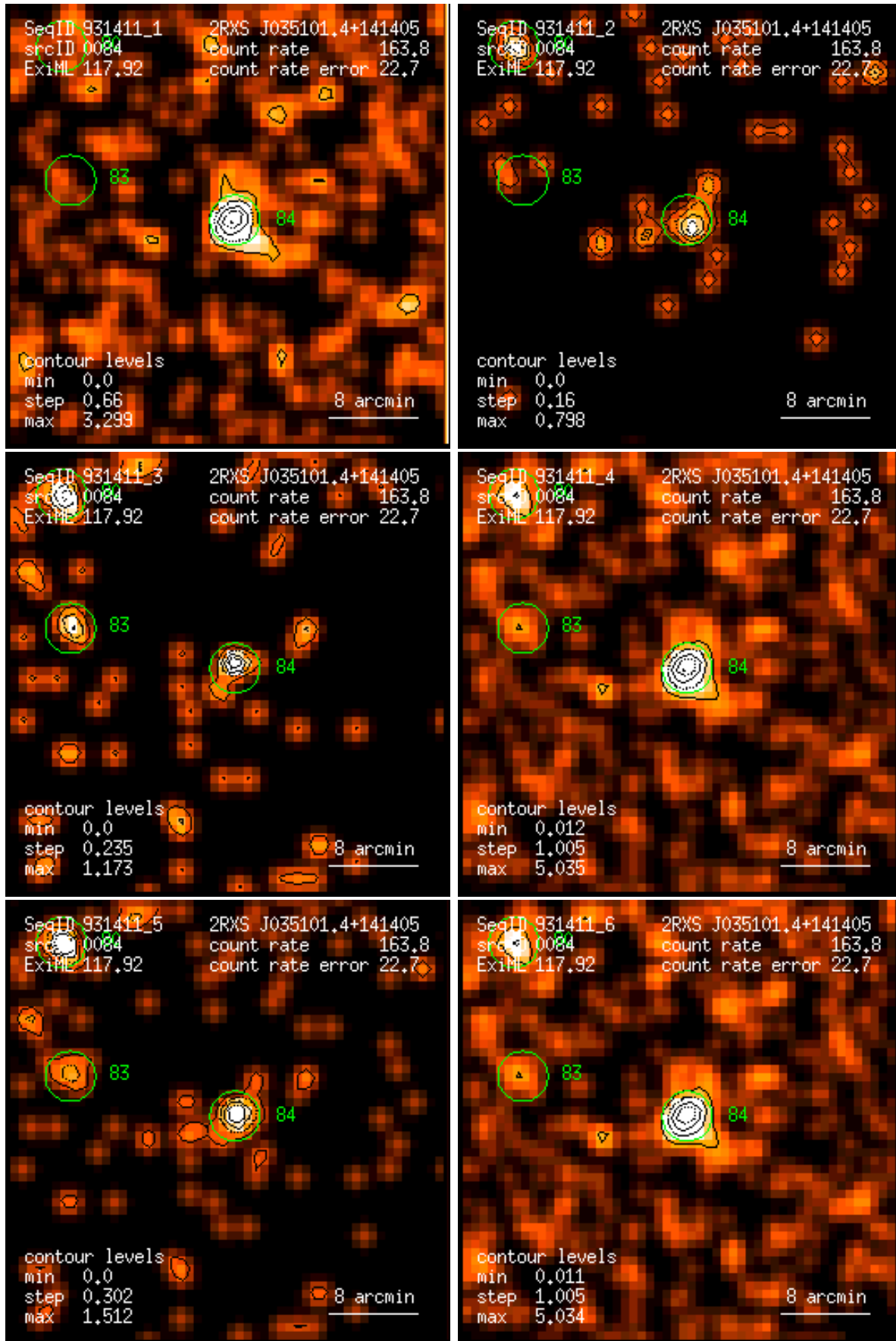
Figure 84: RASS 931411: detection 0084: band rate images, Gaussian filter: (1) PSPC channels 11 – 41, (2) 52 – 90, (3) 91 – 201, (4) 11 – 235, (5) 52 – 201, (6) 11 – 201. Broad band rates in counts/ks. Band rate contour levels in counts/ks/arcmin 2 .
