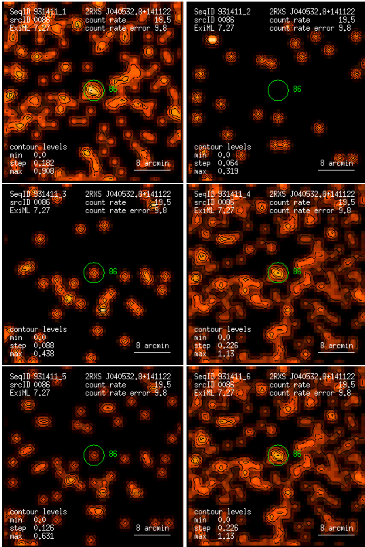
Figure 86: RASS 931411: detection 0086: band rate images, Gaussian filter: (1) PSPC channels 11 – 41, (2) 52 – 90, (3) 91 – 201, (4) 11 – 235, (5) 52 – 201, (6) 11 – 201. Broad band rates in counts/ks. Band rate contour levels in counts/ks/arcmin 2 .
