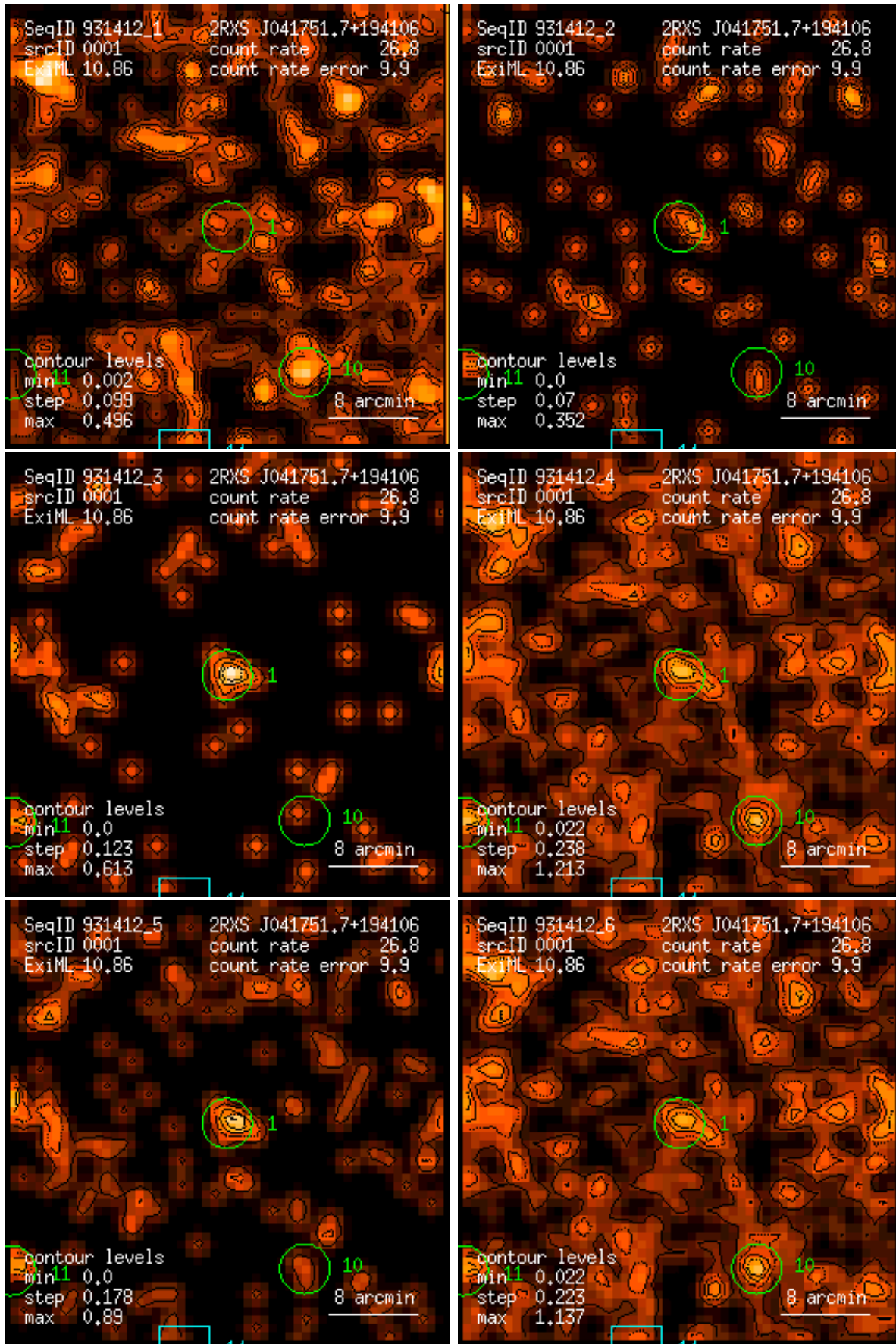
Figure 1: RASS 931412: detection 0001: band rate images, Gaussian filter: (1) PSPC channels 11 – 41, (2) 52 – 90, (3) 91 – 201, (4) 11 – 235, (5) 52 – 201, (6) 11 – 201. Broad band rates in counts/ks. Band rate contour levels in counts/ks/arcmin 2 .
