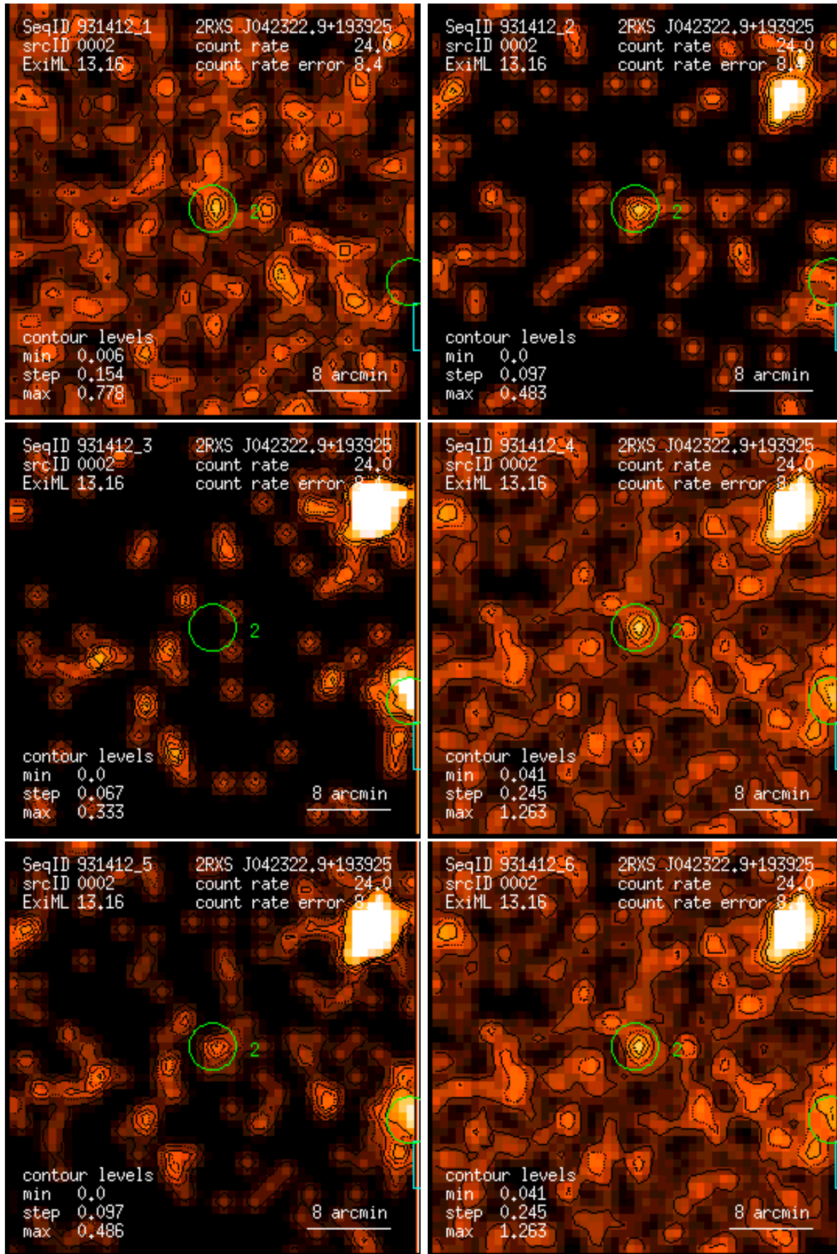
Figure 2: RASS 931412: detection 0002: band rate images, Gaussian filter: (1) PSPC channels 11 – 41, (2) 52 – 90, (3) 91 – 201, (4) 11 – 235, (5) 52 – 201, (6) 11 – 201. Broad band rates in counts/ks. Band rate contour levels in counts/ks/arcmin 2 .
