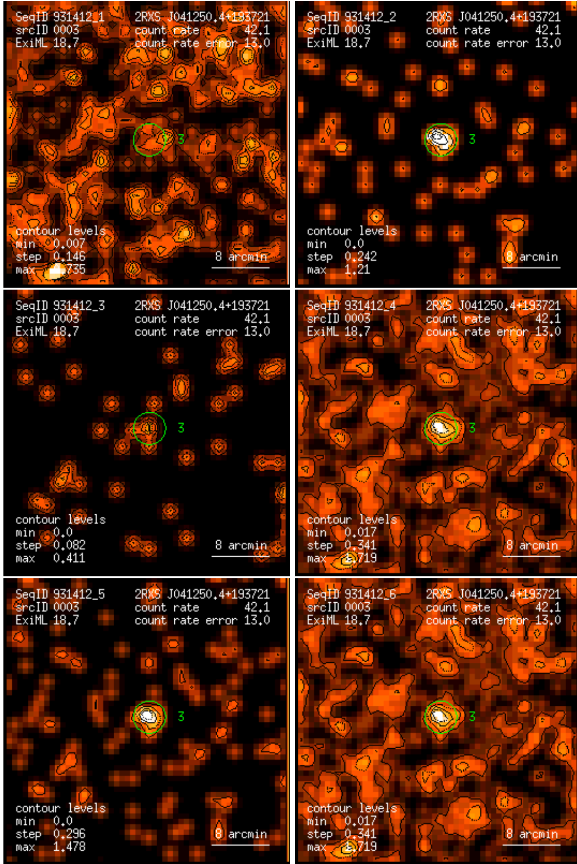
Figure 3: RASS 931412: detection 0003: band rate images, Gaussian filter: (1) PSPC channels 11 – 41, (2) 52 – 90, (3) 91 – 201, (4) 11 – 235, (5) 52 – 201, (6) 11 – 201. Broad band rates in counts/ks. Band rate contour levels in counts/ks/arcmin 2 .
