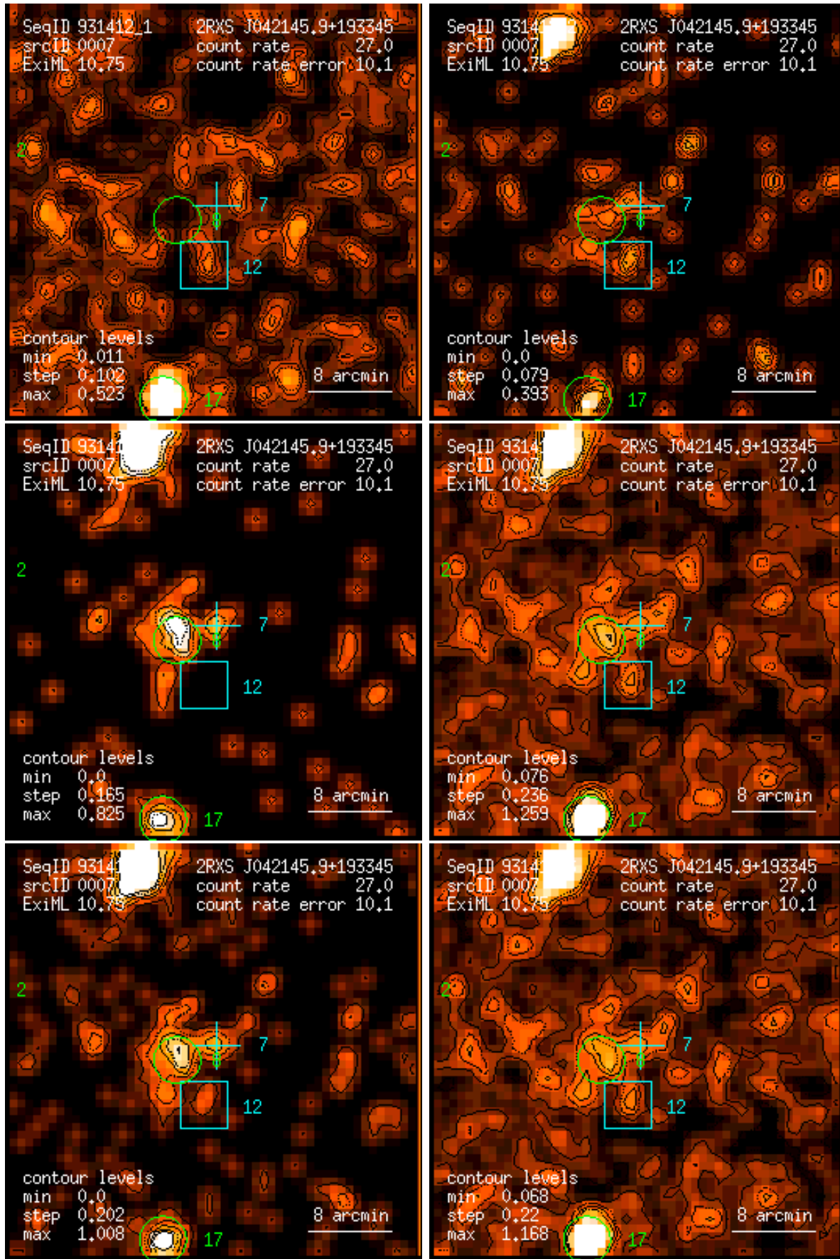
Figure 7: RASS 931412: detection 0007: band rate images, Gaussian filter: (1) PSPC channels 11 – 41, (2) 52 – 90, (3) 91 – 201, (4) 11 – 235, (5) 52 – 201, (6) 11 – 201. Broad band rates in counts/ks. Band rate contour levels in counts/ks/arcmin 2 .
