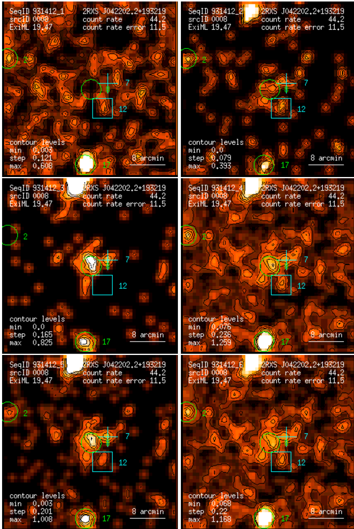
Figure 8: RASS 931412: detection 0008: band rate images, Gaussian filter: (1) PSPC channels 11 – 41, (2) 52 – 90, (3) 91 – 201, (4) 11 – 235, (5) 52 – 201, (6) 11 – 201. Broad band rates in counts/ks. Band rate contour levels in counts/ks/arcmin 2 .
