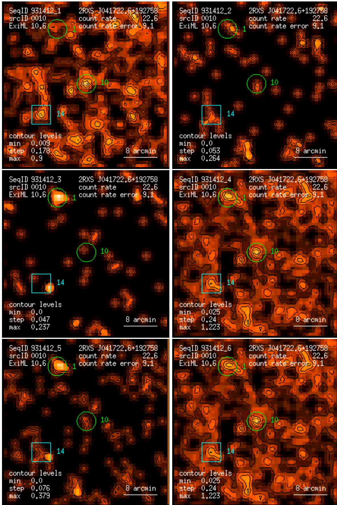
Figure 10: RASS 931412: detection 0010: band rate images, Gaussian filter: (1) PSPC channels 11 – 41, (2) 52 – 90, (3) 91 – 201, (4) 11 – 235, (5) 52 – 201, (6) 11 – 201. Broad band rates in counts/ks. Band rate contour levels in counts/ks/arcmin 2 .
