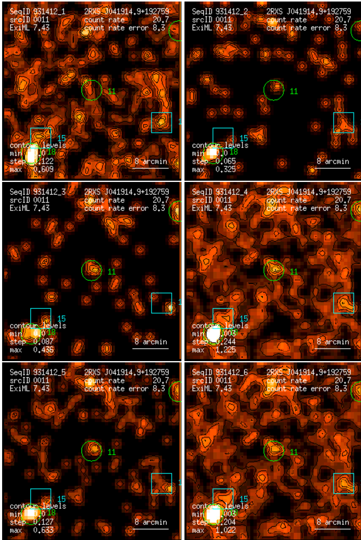
Figure 11: RASS 931412: detection 0011: band rate images, Gaussian filter: (1) PSPC channels 11 – 41, (2) 52 – 90, (3) 91 – 201, (4) 11 – 235, (5) 52 – 201, (6) 11 – 201. Broad band rates in counts/ks. Band rate contour levels in counts/ks/arcmin 2 .
