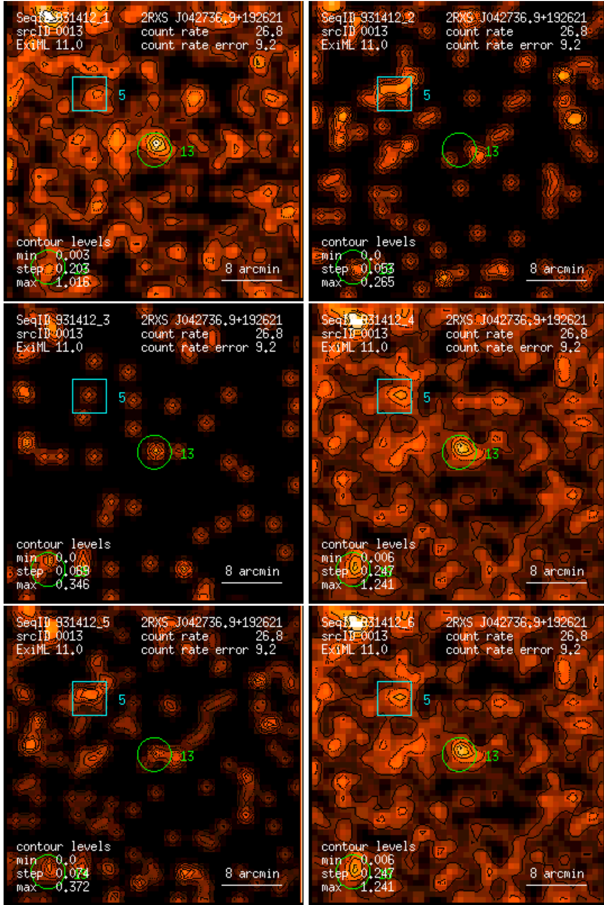
Figure 13: RASS 931412: detection 0013: band rate images, Gaussian filter: (1) PSPC channels 11 – 41, (2) 52 – 90, (3) 91 – 201, (4) 11 – 235, (5) 52 – 201, (6) 11 – 201. Broad band rates in counts/ks. Band rate contour levels in counts/ks/arcmin 2 .
