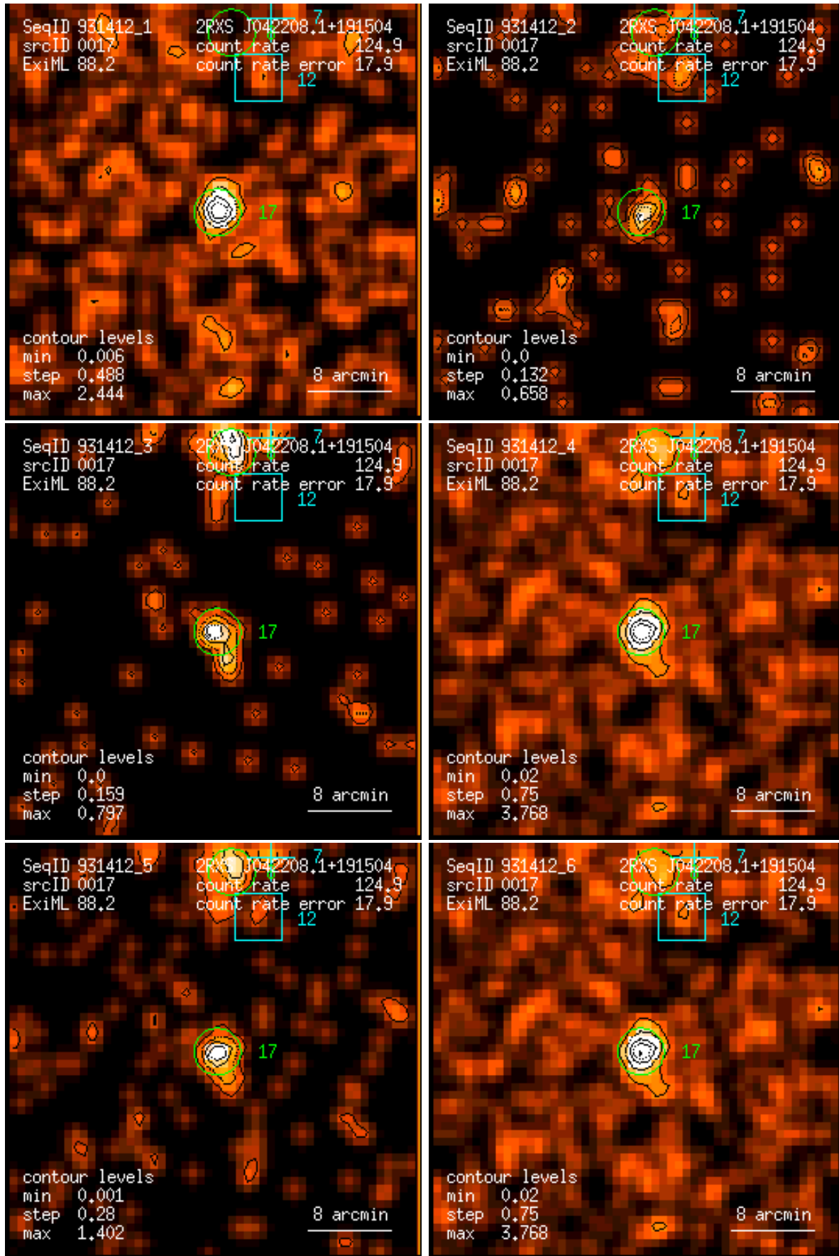
Figure 17: RASS 931412: detection 0017: band rate images, Gaussian filter: (1) PSPC channels 11 – 41, (2) 52 – 90, (3) 91 – 201, (4) 11 – 235, (5) 52 – 201, (6) 11 – 201. Broad band rates in counts/ks. Band rate contour levels in counts/ks/arcmin 2 .
