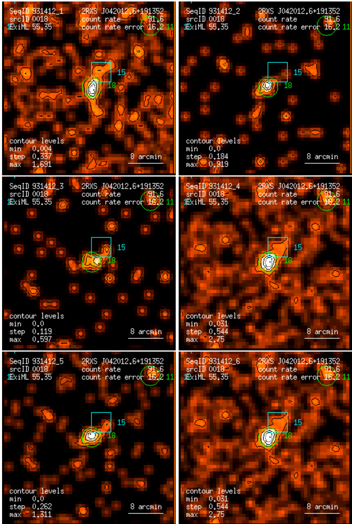
Figure 18: RASS 931412: detection 0018: band rate images, Gaussian filter: (1) PSPC channels 11 – 41, (2) 52 – 90, (3) 91 – 201, (4) 11 – 235, (5) 52 – 201, (6) 11 – 201. Broad band rates in counts/ks. Band rate contour levels in counts/ks/arcmin 2 .
