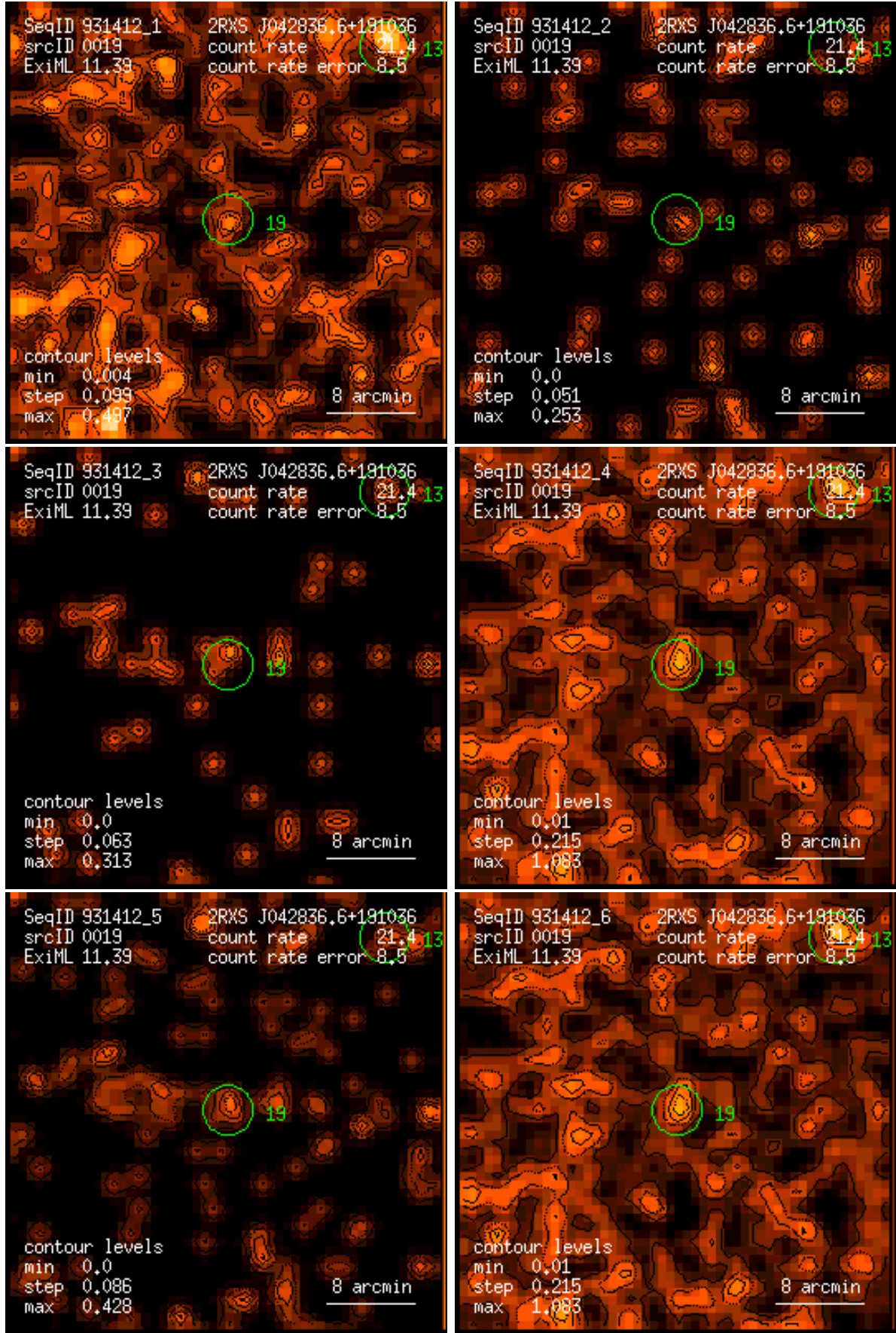
Figure 19: RASS 931412: detection 0019: band rate images, Gaussian filter: (1) PSPC channels 11 – 41, (2) 52 – 90, (3) 91 – 201, (4) 11 – 235, (5) 52 – 201, (6) 11 – 201. Broad band rates in counts/ks. Band rate contour levels in counts/ks/arcmin 2 .
