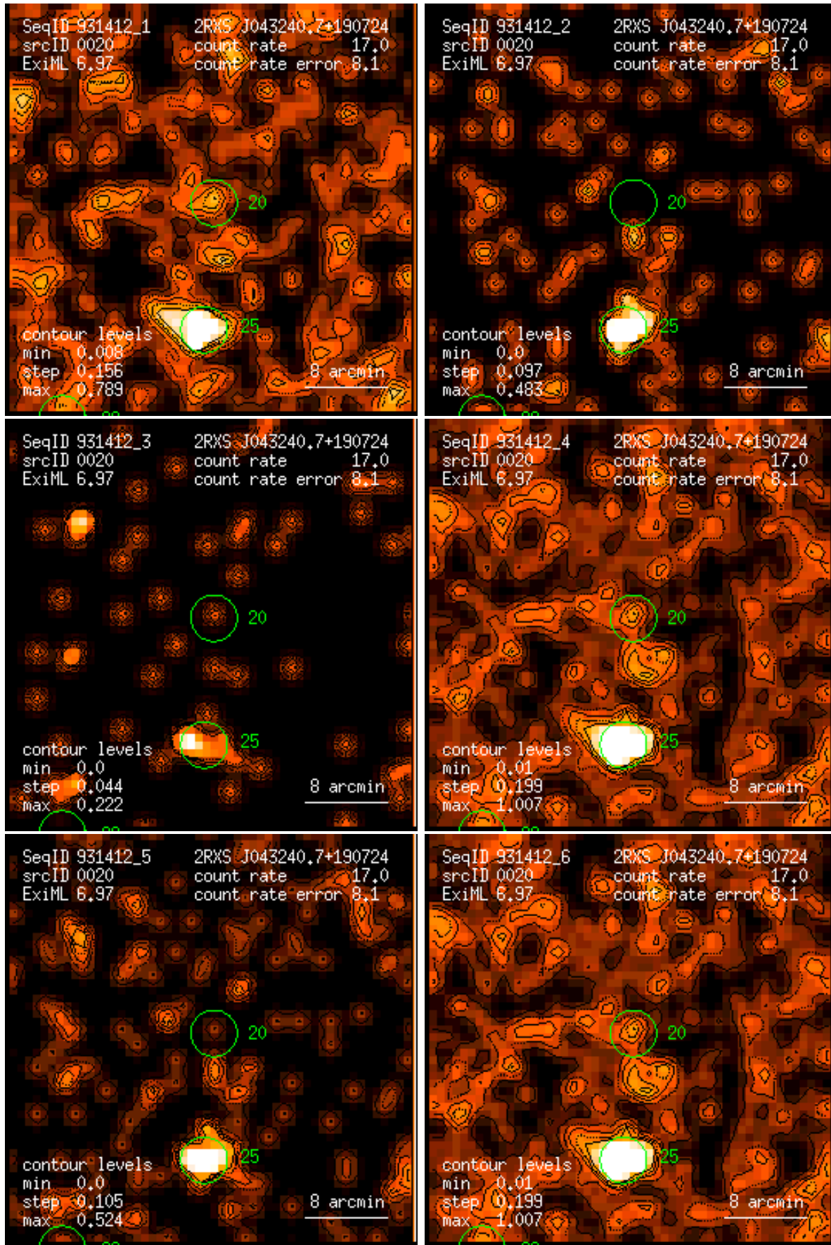
Figure 20: RASS 931412: detection 0020: band rate images, Gaussian filter: (1) PSPC channels 11 – 41, (2) 52 – 90, (3) 91 – 201, (4) 11 – 235, (5) 52 – 201, (6) 11 – 201. Broad band rates in counts/ks. Band rate contour levels in counts/ks/arcmin 2 .
