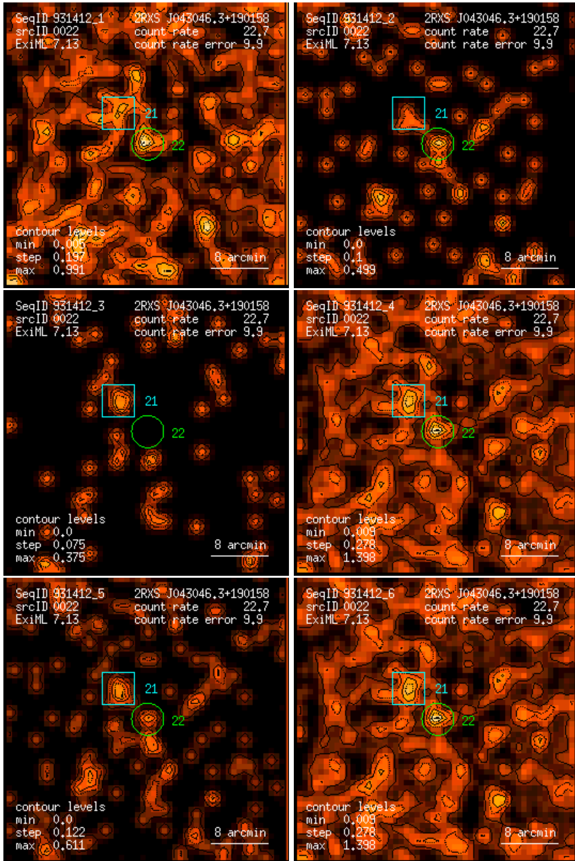
Figure 22: RASS 931412: detection 0022: band rate images, Gaussian filter: (1) PSPC channels 11 – 41, (2) 52 – 90, (3) 91 – 201, (4) 11 – 235, (5) 52 – 201, (6) 11 – 201. Broad band rates in counts/ks. Band rate contour levels in counts/ks/arcmin 2 .
