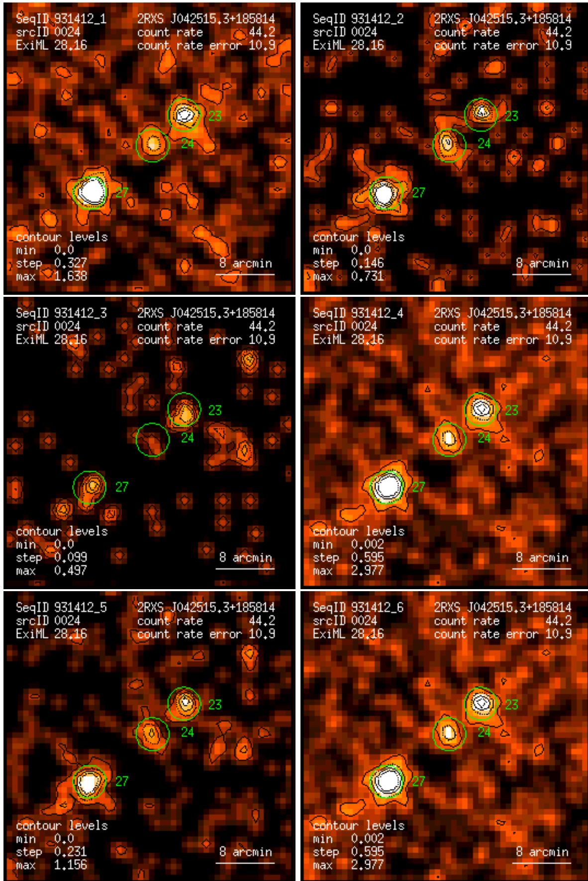
Figure 24: RASS 931412: detection 0024: band rate images, Gaussian filter: (1) PSPC channels 11 – 41, (2) 52 – 90, (3) 91 – 201, (4) 11 – 235, (5) 52 – 201, (6) 11 – 201. Broad band rates in counts/ks. Band rate contour levels in counts/ks/arcmin 2 .
