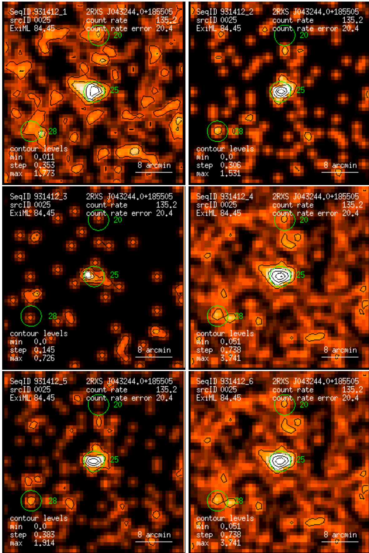
Figure 25: RASS 931412: detection 0025: band rate images, Gaussian filter: (1) PSPC channels 11 – 41, (2) 52 – 90, (3) 91 – 201, (4) 11 – 235, (5) 52 – 201, (6) 11 – 201. Broad band rates in counts/ks. Band rate contour levels in counts/ks/arcmin 2 .
