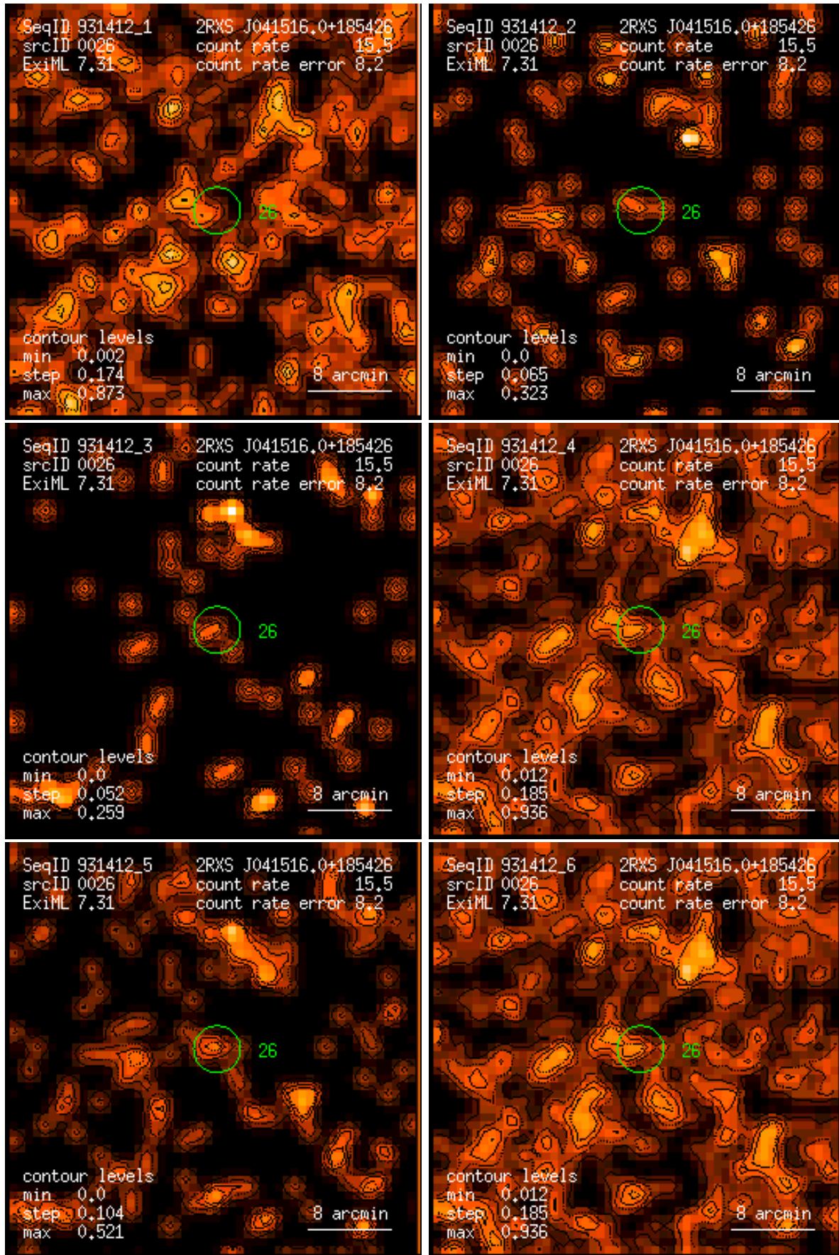
Figure 26: RASS 931412: detection 0026: band rate images, Gaussian filter: (1) PSPC channels 11 – 41, (2) 52 – 90, (3) 91 – 201, (4) 11 – 235, (5) 52 – 201, (6) 11 – 201. Broad band rates in counts/ks. Band rate contour levels in counts/ks/arcmin 2 .
