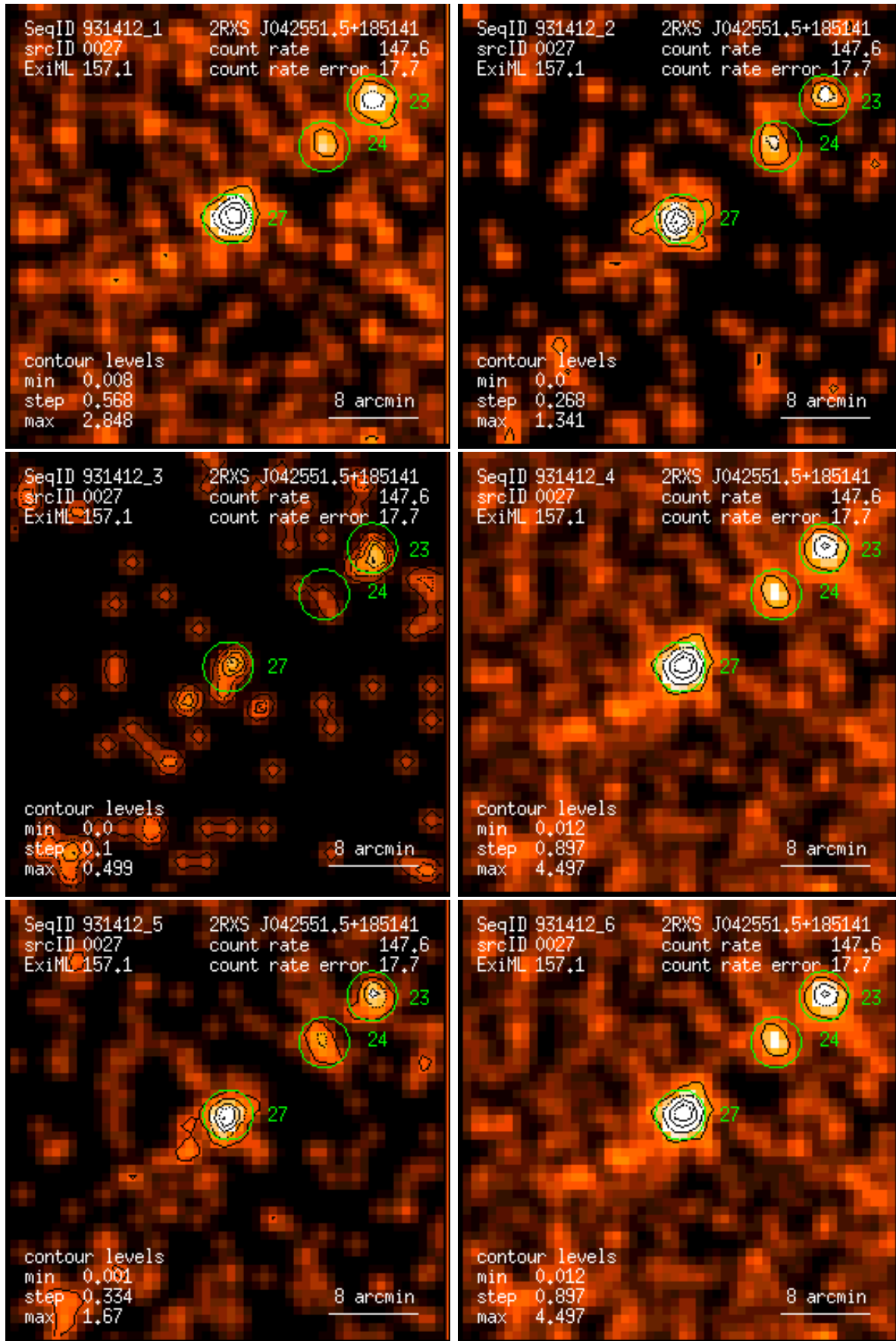
Figure 27: RASS 931412: detection 0027: band rate images, Gaussian filter: (1) PSPC channels 11 – 41, (2) 52 – 90, (3) 91 – 201, (4) 11 – 235, (5) 52 – 201, (6) 11 – 201. Broad band rates in counts/ks. Band rate contour levels in counts/ks/arcmin 2 .
