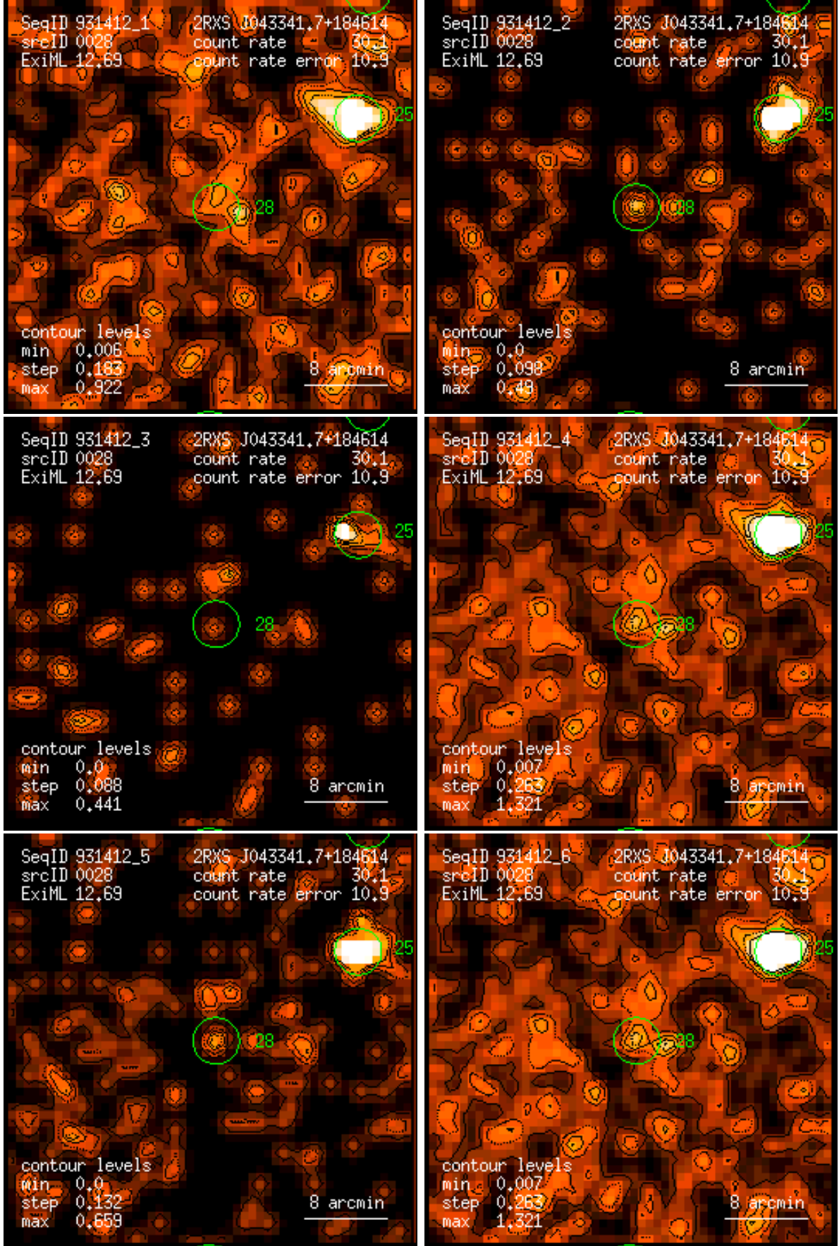
Figure 28: RASS 931412: detection 0028: band rate images, Gaussian filter: (1) PSPC channels 11 – 41, (2) 52 – 90, (3) 91 – 201, (4) 11 – 235, (5) 52 – 201, (6) 11 – 201. Broad band rates in counts/ks. Band rate contour levels in counts/ks/arcmin 2 .
