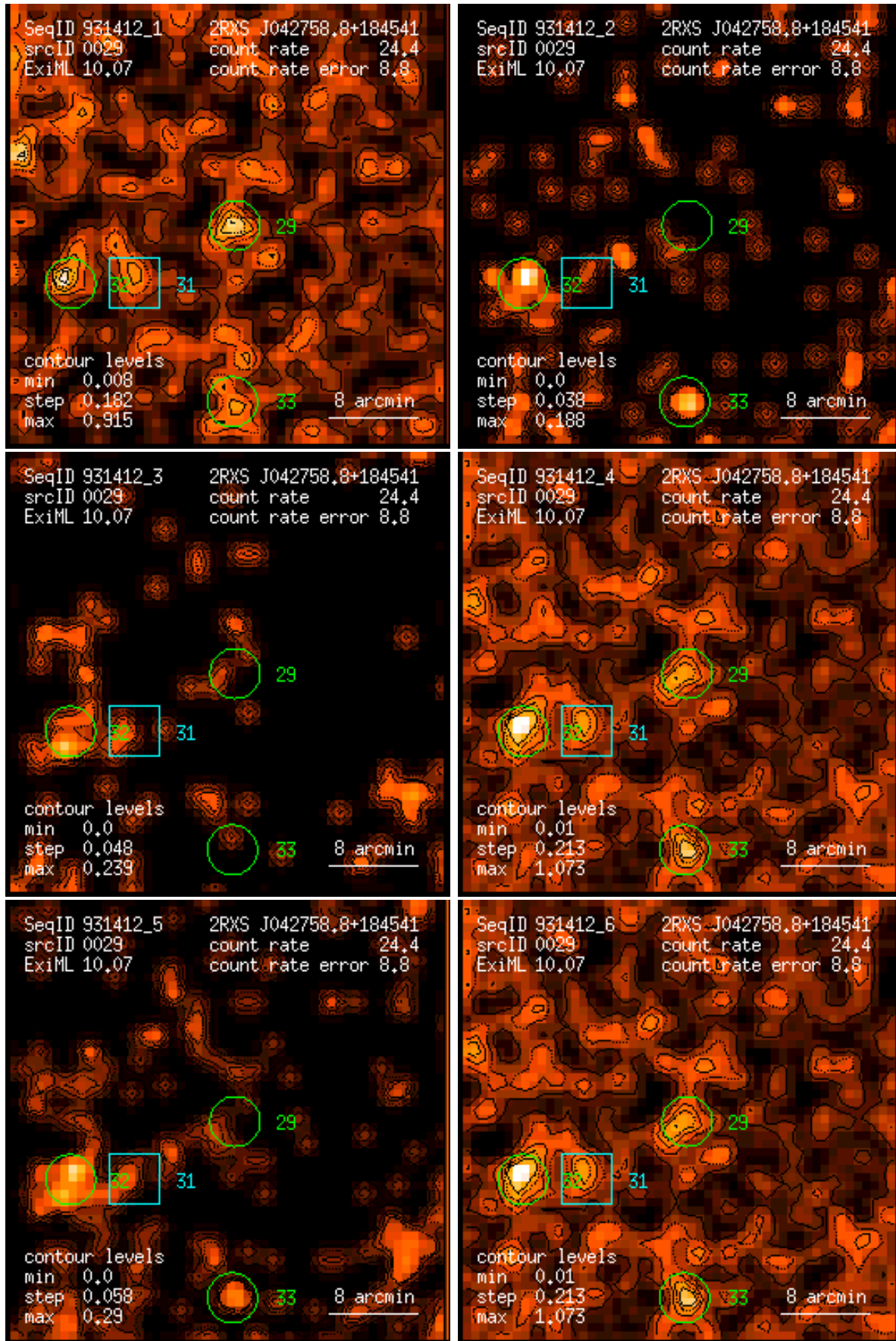
Figure 29: RASS 931412: detection 0029: band rate images, Gaussian filter: (1) PSPC channels 11 – 41, (2) 52 – 90, (3) 91 – 201, (4) 11 – 235, (5) 52 – 201, (6) 11 – 201. Broad band rates in counts/ks. Band rate contour levels in counts/ks/arcmin 2 .
