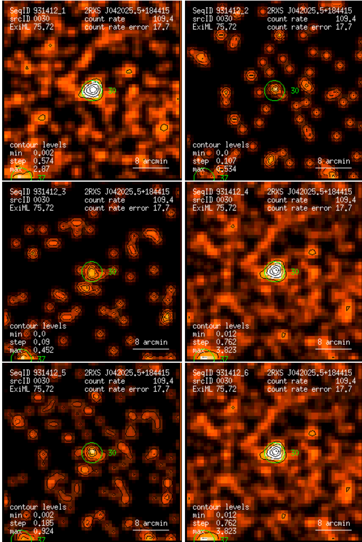
Figure 30: RASS 931412: detection 0030: band rate images, Gaussian filter: (1) PSPC channels 11 – 41, (2) 52 – 90, (3) 91 – 201, (4) 11 – 235, (5) 52 – 201, (6) 11 – 201. Broad band rates in counts/ks. Band rate contour levels in counts/ks/arcmin 2 .
