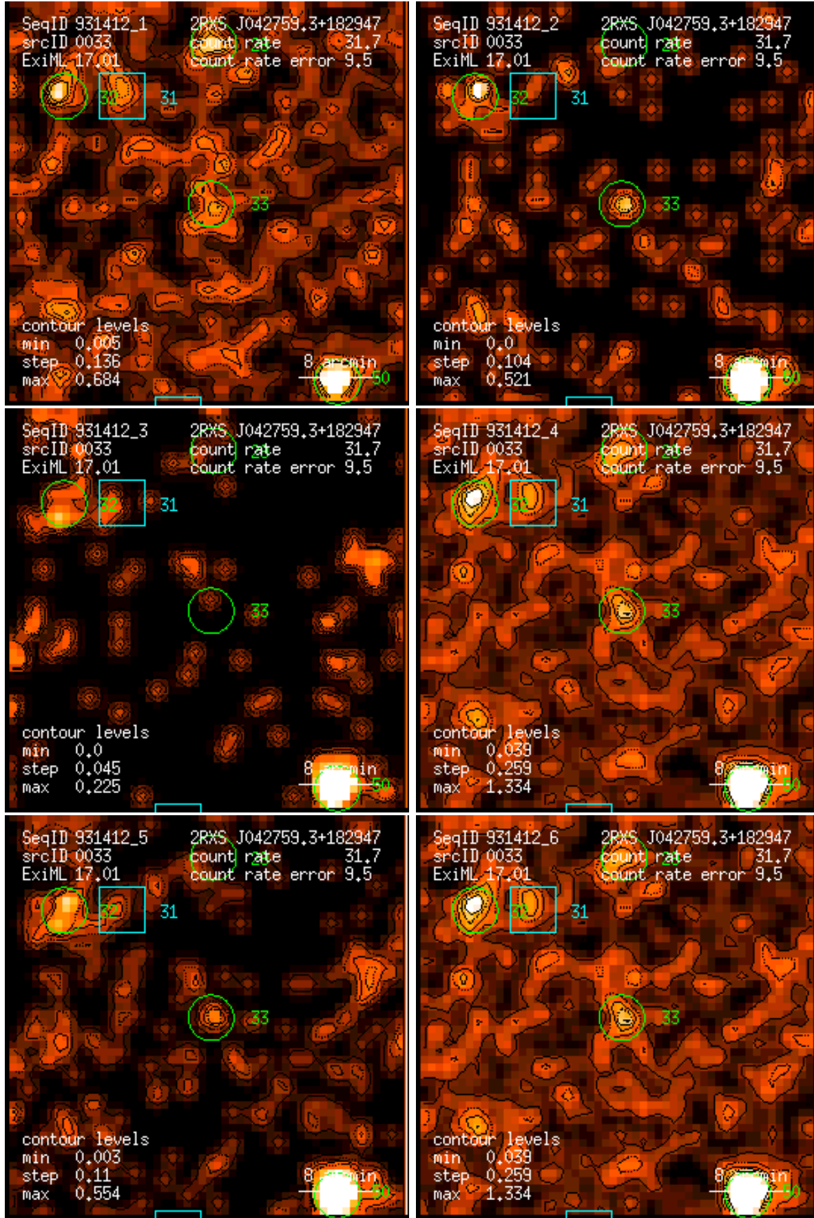
Figure 33: RASS 931412: detection 0033: band rate images, Gaussian filter: (1) PSPC channels 11 – 41, (2) 52 – 90, (3) 91 – 201, (4) 11 – 235, (5) 52 – 201, (6) 11 – 201. Broad band rates in counts/ks. Band rate contour levels in counts/ks/arcmin 2 .
