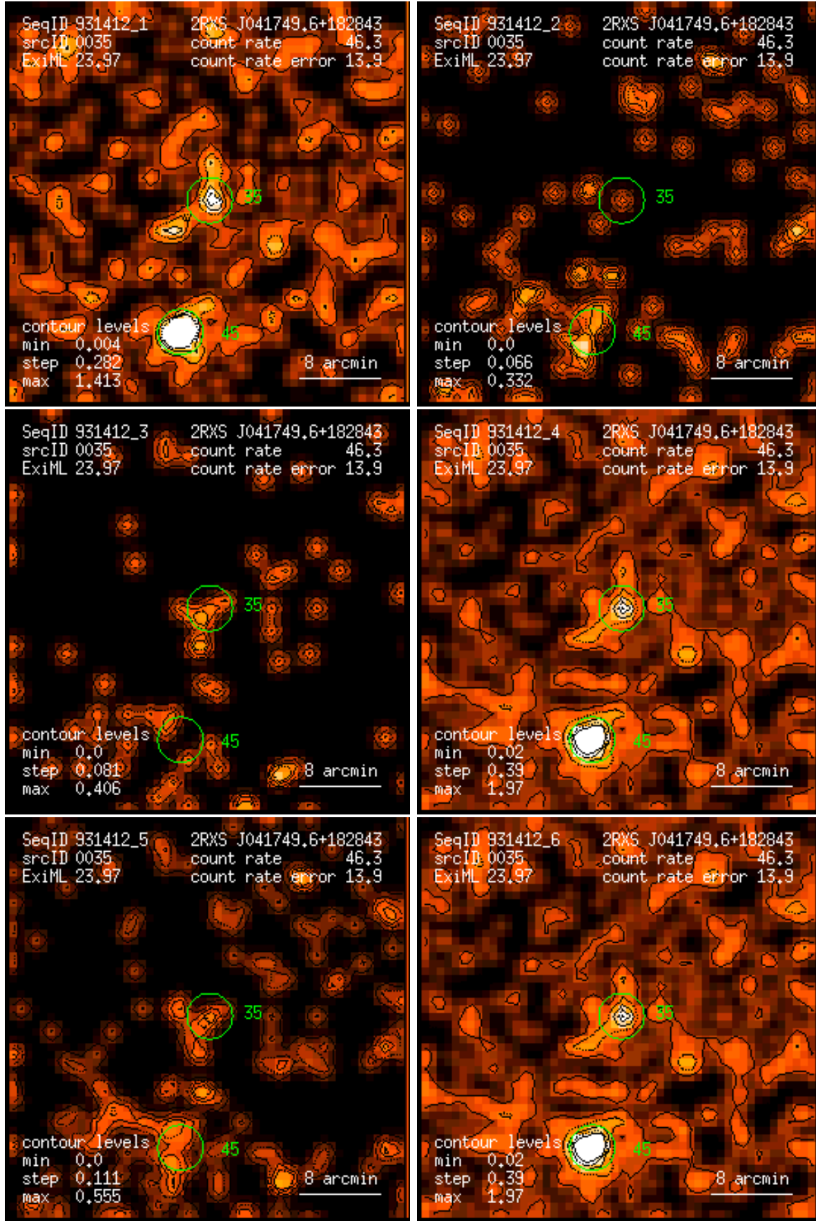
Figure 35: RASS 931412: detection 0035: band rate images, Gaussian filter: (1) PSPC channels 11 – 41, (2) 52 – 90, (3) 91 – 201, (4) 11 – 235, (5) 52 – 201, (6) 11 – 201. Broad band rates in counts/ks. Band rate contour levels in counts/ks/arcmin 2 .
