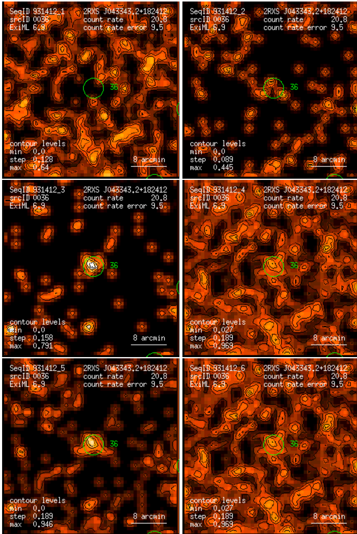
Figure 36: RASS 931412: detection 0036: band rate images, Gaussian filter: (1) PSPC channels 11 – 41, (2) 52 – 90, (3) 91 – 201, (4) 11 – 235, (5) 52 – 201, (6) 11 – 201. Broad band rates in counts/ks. Band rate contour levels in counts/ks/arcmin 2 .
