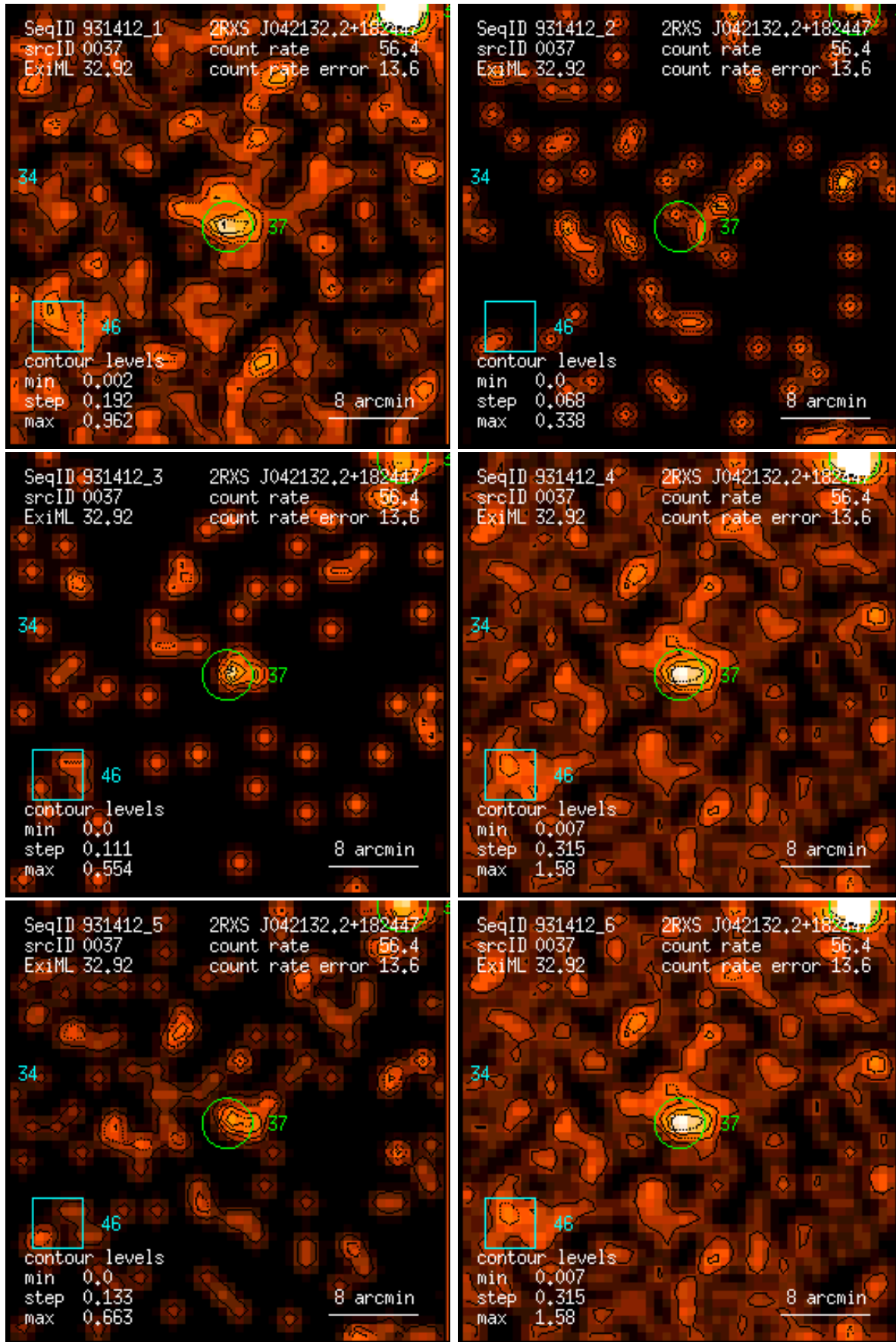
Figure 37: RASS 931412: detection 0037: band rate images, Gaussian filter: (1) PSPC channels 11 – 41, (2) 52 – 90, (3) 91 – 201, (4) 11 – 235, (5) 52 – 201, (6) 11 – 201. Broad band rates in counts/ks. Band rate contour levels in counts/ks/arcmin 2 .
