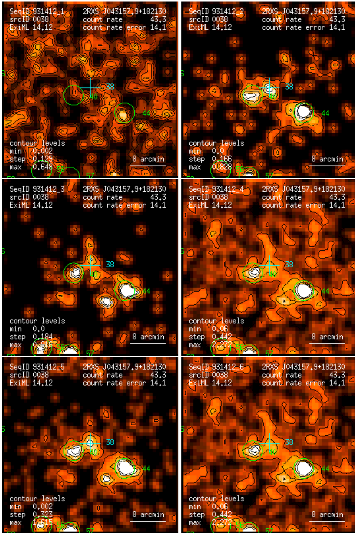
Figure 38: RASS 931412: detection 0038: band rate images, Gaussian filter: (1) PSPC channels 11 – 41, (2) 52 – 90, (3) 91 – 201, (4) 11 – 235, (5) 52 – 201, (6) 11 – 201. Broad band rates in counts/ks. Band rate contour levels in counts/ks/arcmin 2 .
