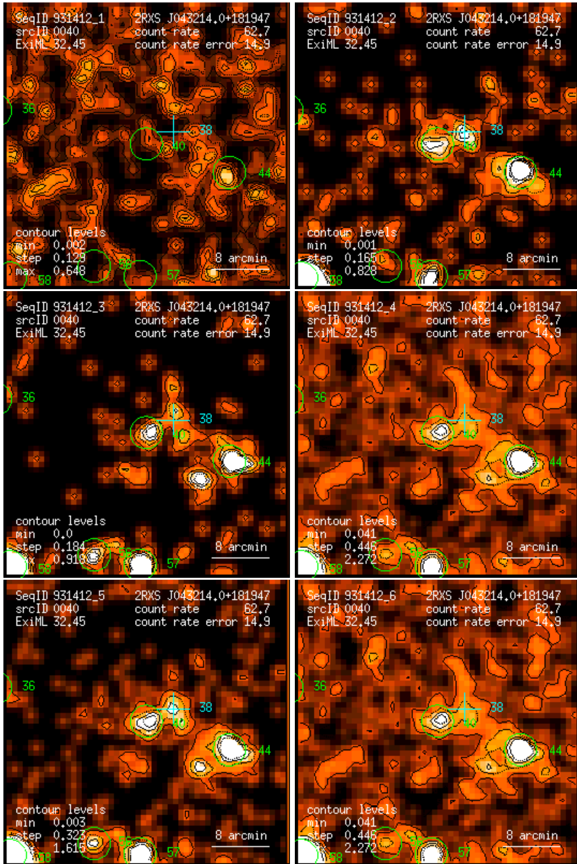
Figure 40: RASS 931412: detection 0040: band rate images, Gaussian filter: (1) PSPC channels 11 – 41, (2) 52 – 90, (3) 91 – 201, (4) 11 – 235, (5) 52 – 201, (6) 11 – 201. Broad band rates in counts/ks. Band rate contour levels in counts/ks/arcmin 2 .
