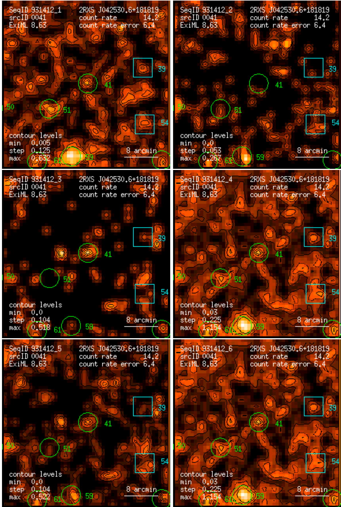
Figure 41: RASS 931412: detection 0041: band rate images, Gaussian filter: (1) PSPC channels 11 – 41, (2) 52 – 90, (3) 91 – 201, (4) 11 – 235, (5) 52 – 201, (6) 11 – 201. Broad band rates in counts/ks. Band rate contour levels in counts/ks/arcmin 2 .
