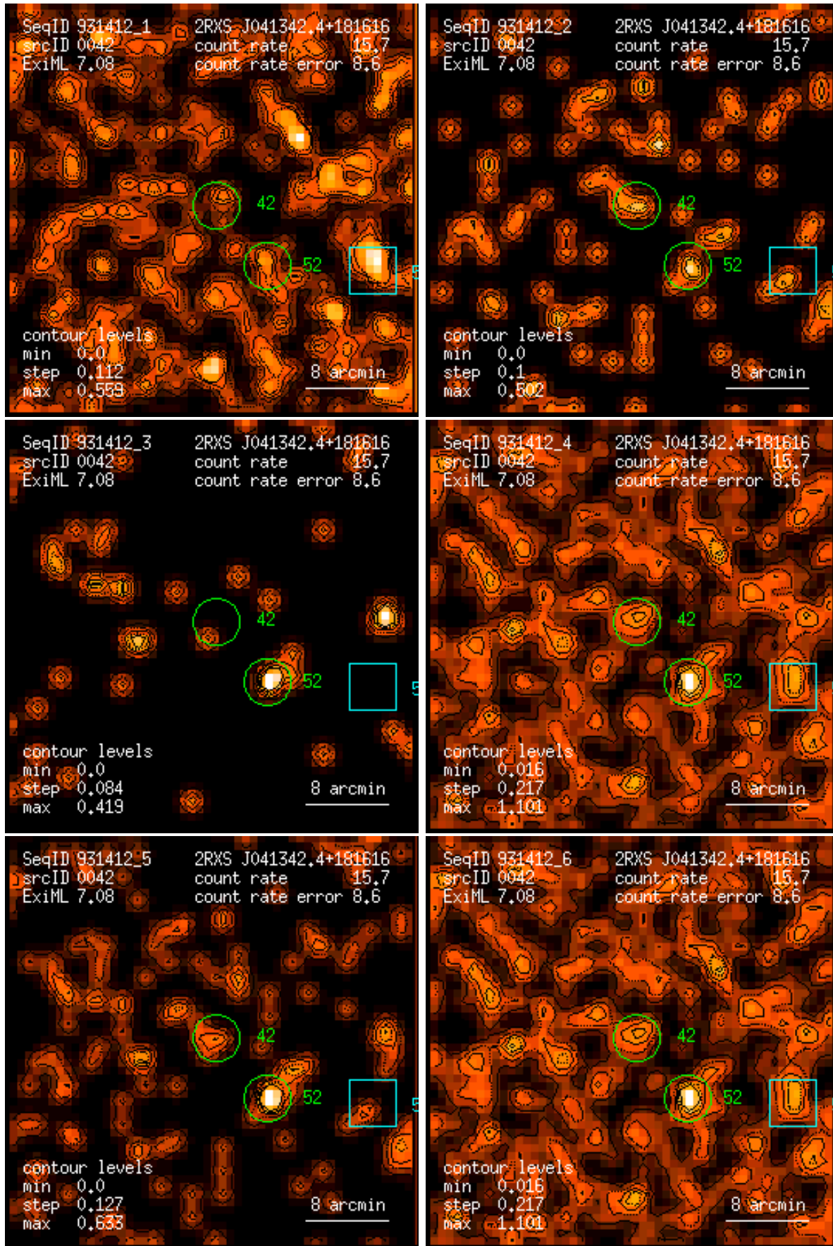
Figure 42: RASS 931412: detection 0042: band rate images, Gaussian filter: (1) PSPC channels 11 – 41, (2) 52 – 90, (3) 91 – 201, (4) 11 – 235, (5) 52 – 201, (6) 11 – 201. Broad band rates in counts/ks. Band rate contour levels in counts/ks/arcmin 2 .
