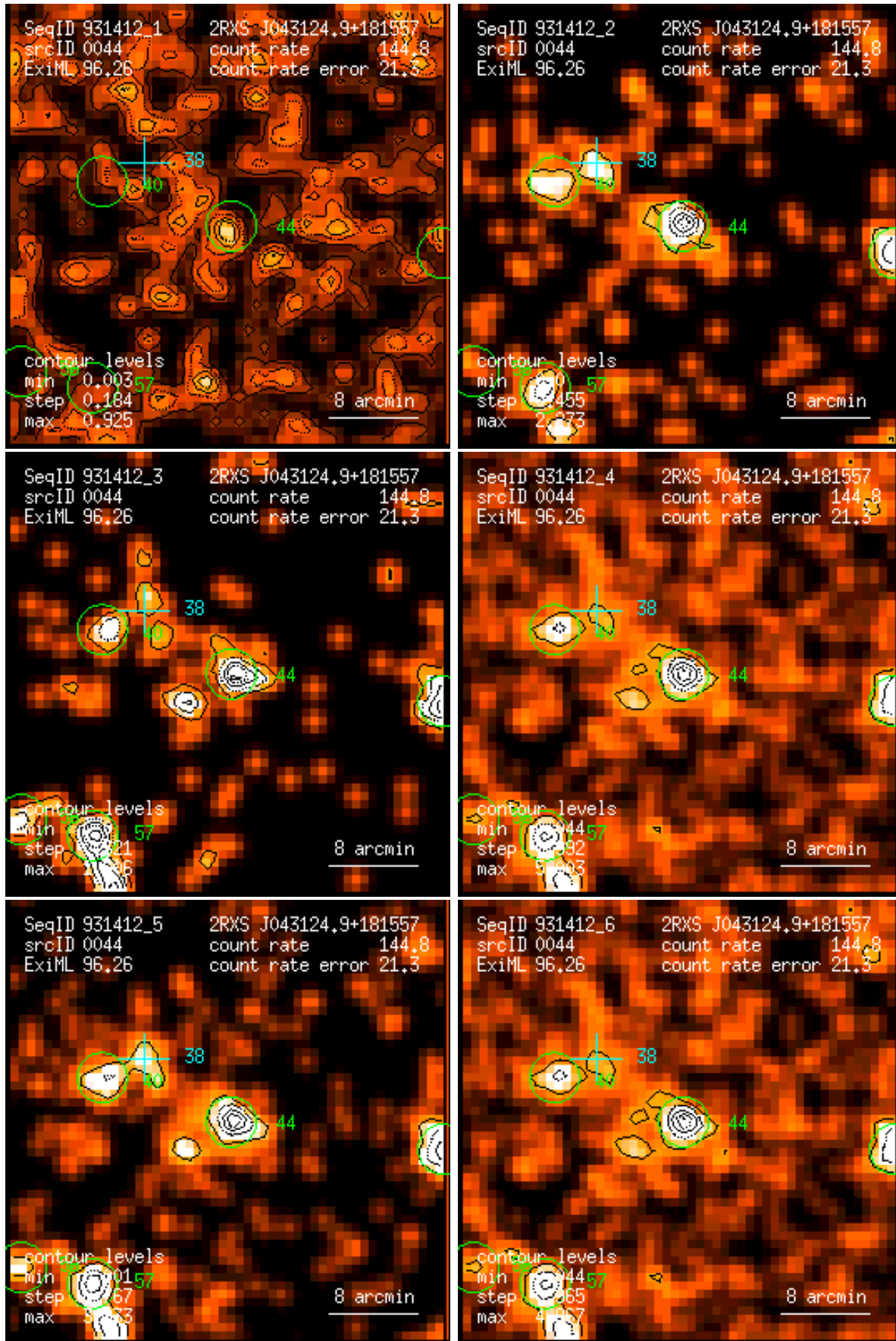
Figure 44: RASS 931412: detection 0044: band rate images, Gaussian filter: (1) PSPC channels 11 – 41, (2) 52 – 90, (3) 91 – 201, (4) 11 – 235, (5) 52 – 201, (6) 11 – 201. Broad band rates in counts/ks. Band rate contour levels in counts/ks/arcmin 2 .
