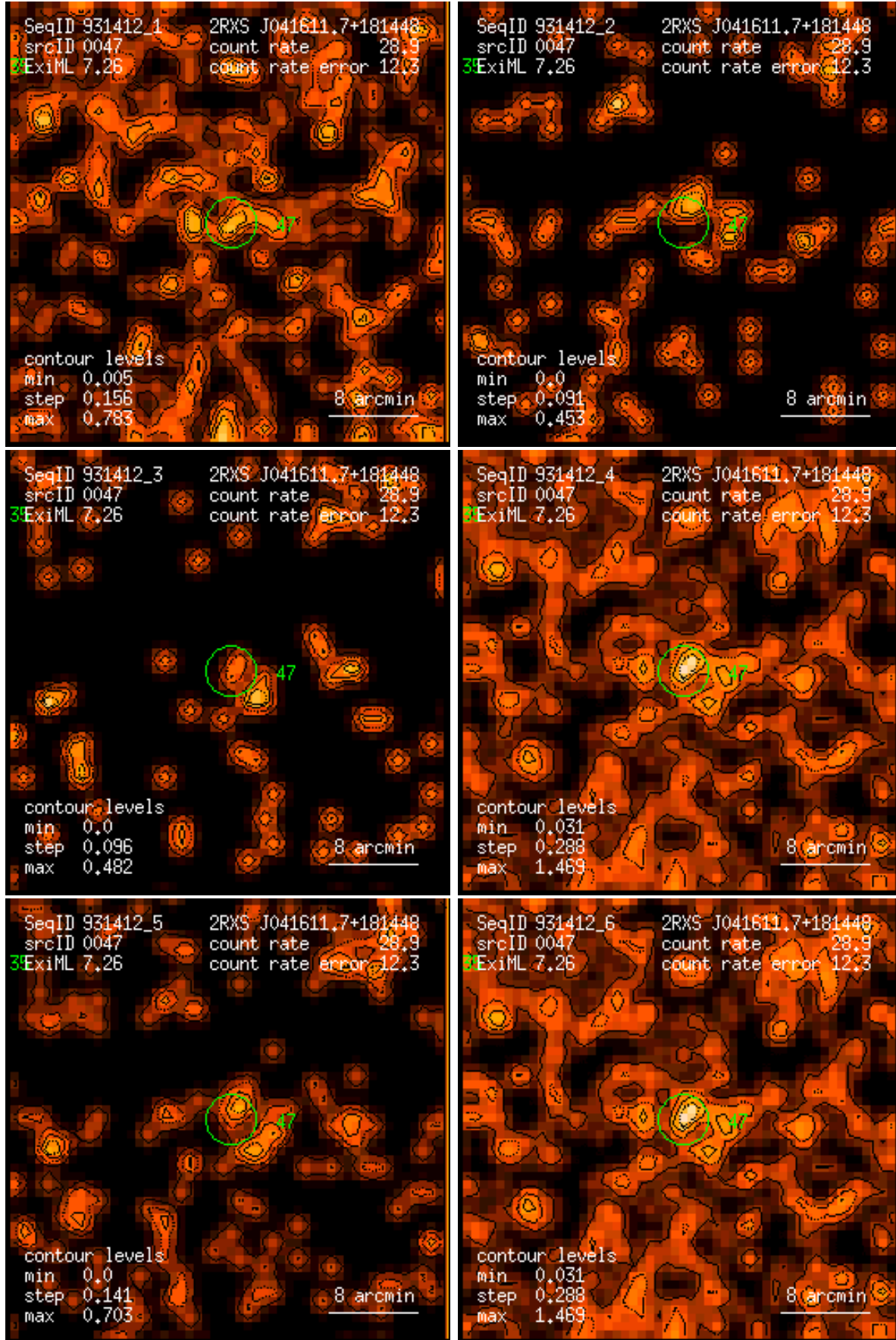
Figure 47: RASS 931412: detection 0047: band rate images, Gaussian filter: (1) PSPC channels 11 – 41, (2) 52 – 90, (3) 91 – 201, (4) 11 – 235, (5) 52 – 201, (6) 11 – 201. Broad band rates in counts/ks. Band rate contour levels in counts/ks/arcmin 2 .
