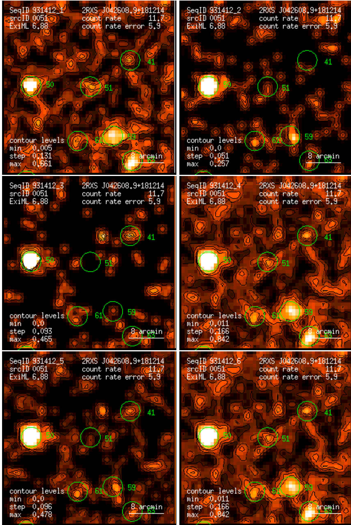
Figure 51: RASS 931412: detection 0051: band rate images, Gaussian filter: (1) PSPC channels 11 – 41, (2) 52 – 90, (3) 91 – 201, (4) 11 – 235, (5) 52 – 201, (6) 11 – 201. Broad band rates in counts/ks. Band rate contour levels in counts/ks/arcmin 2 .
