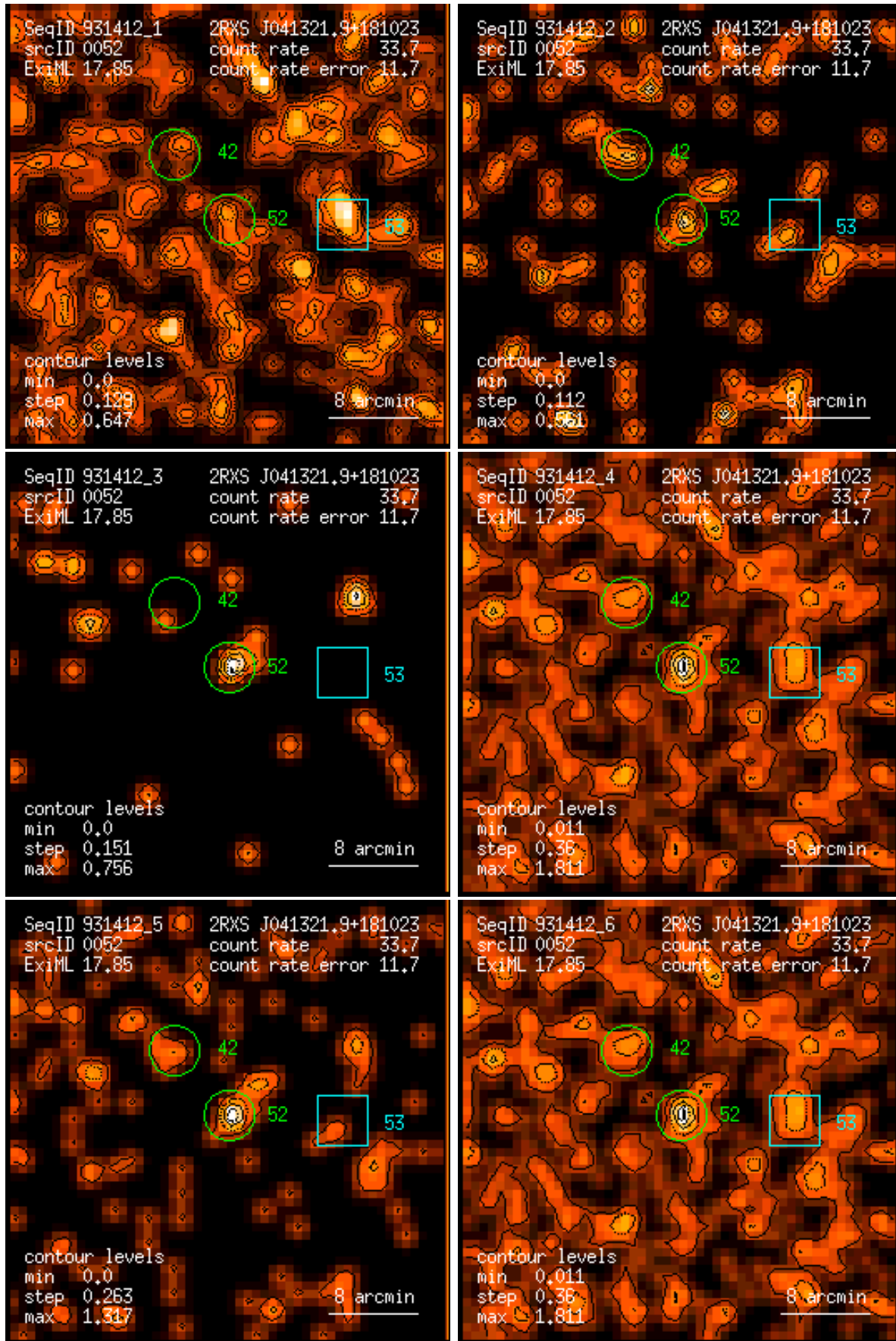
Figure 52: RASS 931412: detection 0052: band rate images, Gaussian filter: (1) PSPC channels 11 – 41, (2) 52 – 90, (3) 91 – 201, (4) 11 – 235, (5) 52 – 201, (6) 11 – 201. Broad band rates in counts/ks. Band rate contour levels in counts/ks/arcmin 2 .
