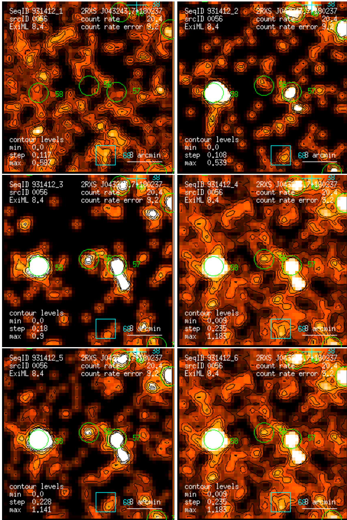
Figure 56: RASS 931412: detection 0056: band rate images, Gaussian filter: (1) PSPC channels 11 – 41, (2) 52 – 90, (3) 91 – 201, (4) 11 – 235, (5) 52 – 201, (6) 11 – 201. Broad band rates in counts/ks. Band rate contour levels in counts/ks/arcmin 2 .
