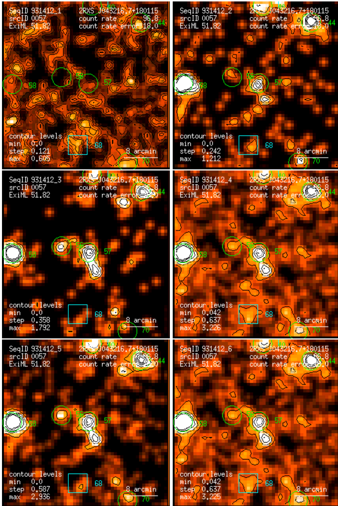
Figure 57: RASS 931412: detection 0057: band rate images, Gaussian filter: (1) PSPC channels 11 – 41, (2) 52 – 90, (3) 91 – 201, (4) 11 – 235, (5) 52 – 201, (6) 11 – 201. Broad band rates in counts/ks. Band rate contour levels in counts/ks/arcmin 2 .
