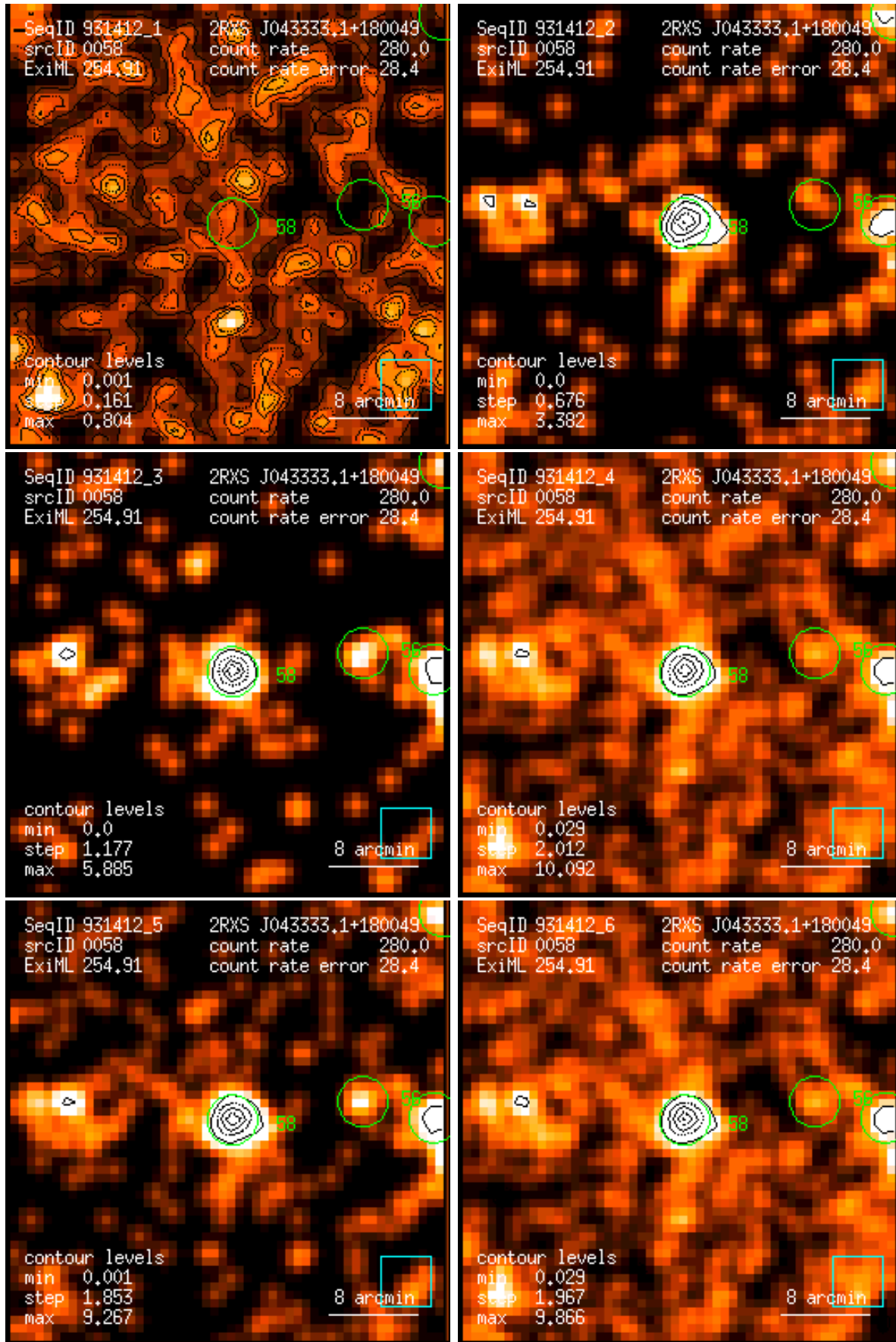
Figure 58: RASS 931412: detection 0058: band rate images, Gaussian filter: (1) PSPC channels 11 – 41, (2) 52 – 90, (3) 91 – 201, (4) 11 – 235, (5) 52 – 201, (6) 11 – 201. Broad band rates in counts/ks. Band rate contour levels in counts/ks/arcmin 2 .
