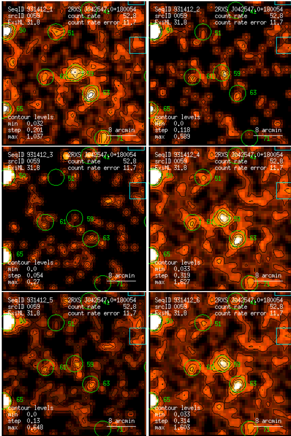
Figure 59: RASS 931412: detection 0059: band rate images, Gaussian filter: (1) PSPC channels 11 – 41, (2) 52 – 90, (3) 91 – 201, (4) 11 – 235, (5) 52 – 201, (6) 11 – 201. Broad band rates in counts/ks. Band rate contour levels in counts/ks/arcmin 2 .
