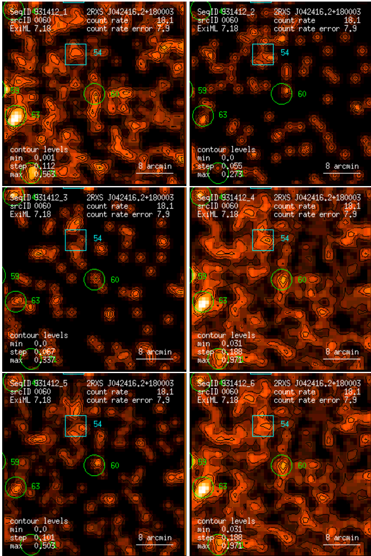
Figure 60: RASS 931412: detection 0060: band rate images, Gaussian filter: (1) PSPC channels 11 – 41, (2) 52 – 90, (3) 91 – 201, (4) 11 – 235, (5) 52 – 201, (6) 11 – 201. Broad band rates in counts/ks. Band rate contour levels in counts/ks/arcmin 2 .
